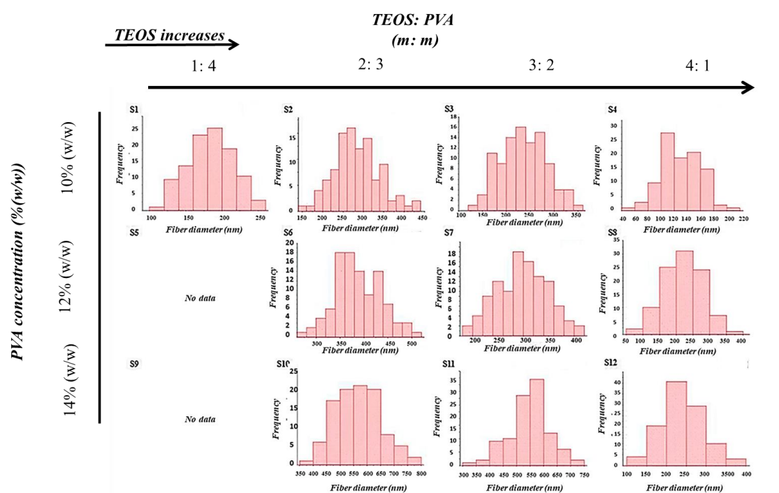
Figure 6. Fiber diameter distribution of the electrospun samples prepared from different tetraethoxysilane (TEOS)/ polyvinyl alcohol (PVA). [IV]
