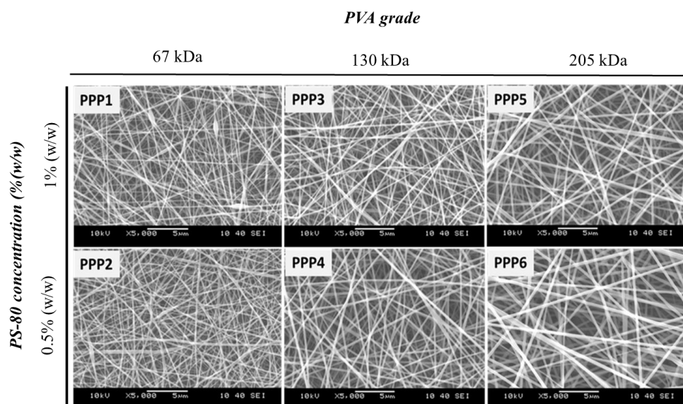
Figure 3. Scanning Electron Microscope (SEM) images of electrospun samples of polyvinyl alcohol (PVA)/poloxamer 407(PO-407) blends with polysorbate 80 (PS-80) (0.5-1% (w/w)), (magnification: 5000 \times ). [IV]
