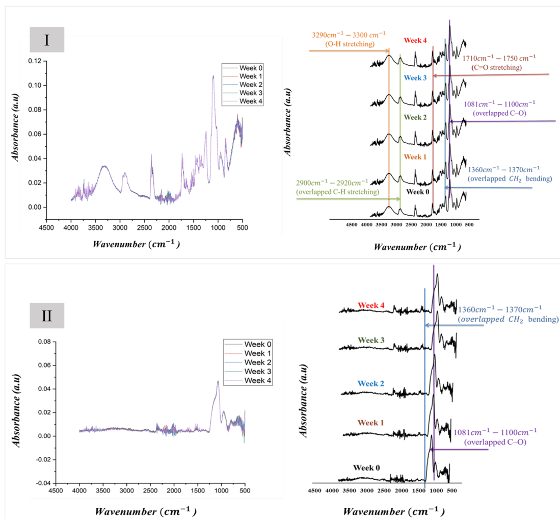
Figure 24. Fourier transform infrared (FTIR) spectra of the cysteamine-loaded (Cys-loaded) fibers at 0, 1-, 2-, 3-, and 4-weeks storage under stress conditions ( 40 \pm 2^\circ\text{C} , 75 \pm 5\% relative humidity (RH)). (I): polyvinyl alcohol (PVA)/poloxamer 407 (PO-407) and (II) tetraetoxysilane (TEOS)/PVA polymeric blends. [IV]
