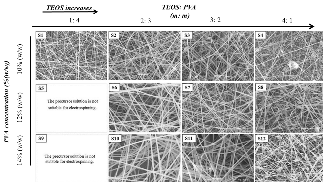
Figure 5. Scanning Electron Microscope (SEM) images of electrospun samples prepared from different composition Tetraethoxysilane (TEOS)/ polyvinyl alcohol (PVA) precursor solutions by electrospinning (Magnification: 3500x). [IV]
