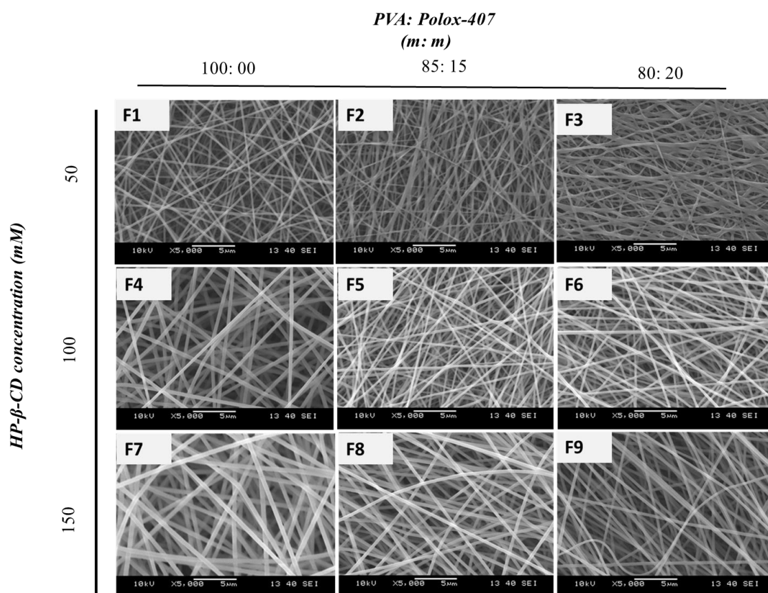
Figure 7. Scanning Electron Microscope (SEM) images of Nepafenac (NEPA)-loaded electrospun samples prepared from nepafenac/ hydroxypropyl-beta-cyclodextrin /polyvinyl alcohol (NEPA/HP- \beta -CD/PVA)(F1, F4, and F7); and NEPA/ HP- \beta -CD/PVA/Poloxamer 407 (F2, F3, F5, F6, F8, and F9) (magnification: 5000 \times ). [III]
