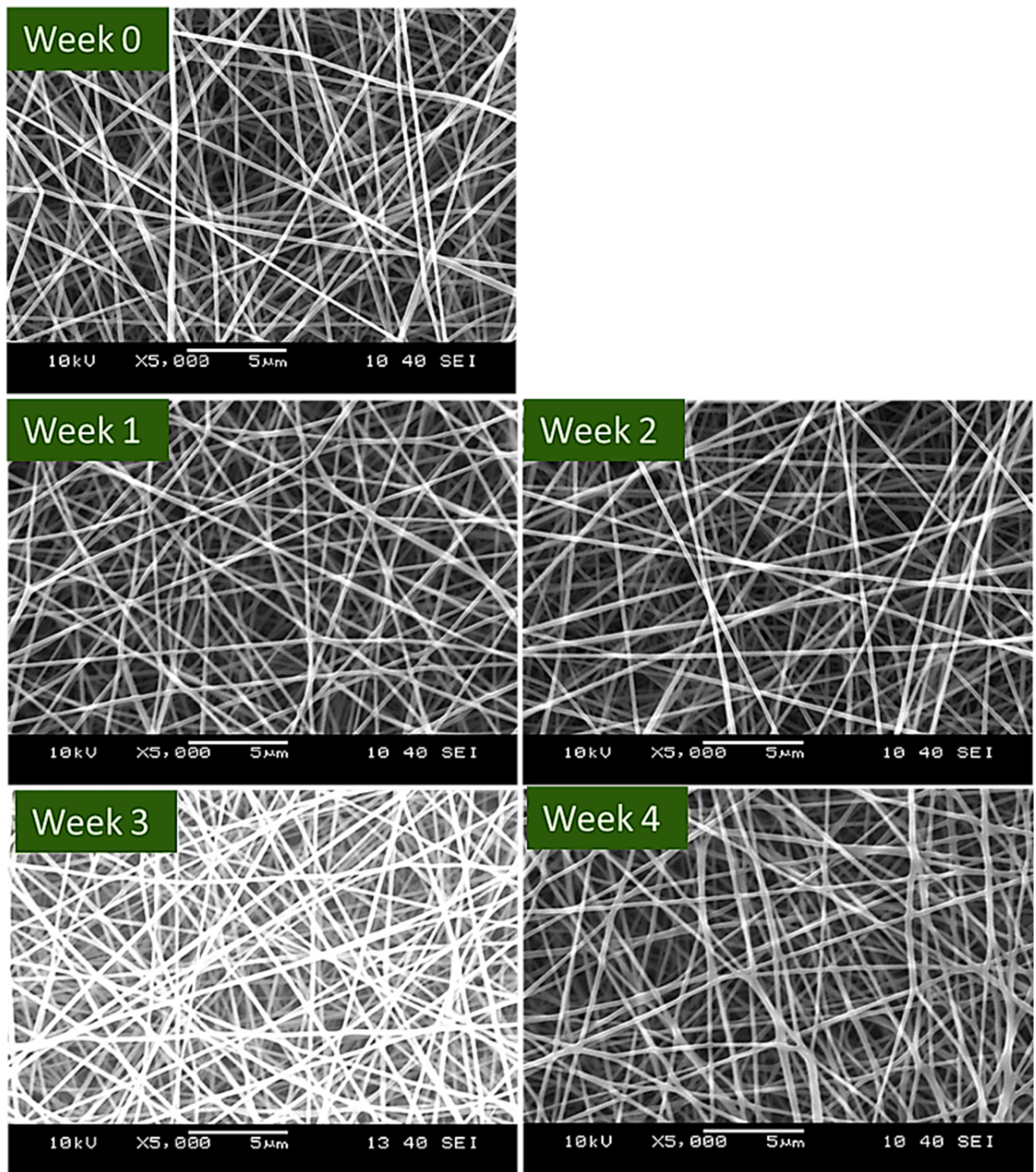
Fig. 9. Scanning electron microscopic (SEM) images of the Nepafenac-loaded fibers at 0, 1, 2, 3, and 4 weeks storage under stress conditions ( 40 \pm 2 °C, 75 \pm 5 % relative humidity). (magnification: 5000 \times ).
