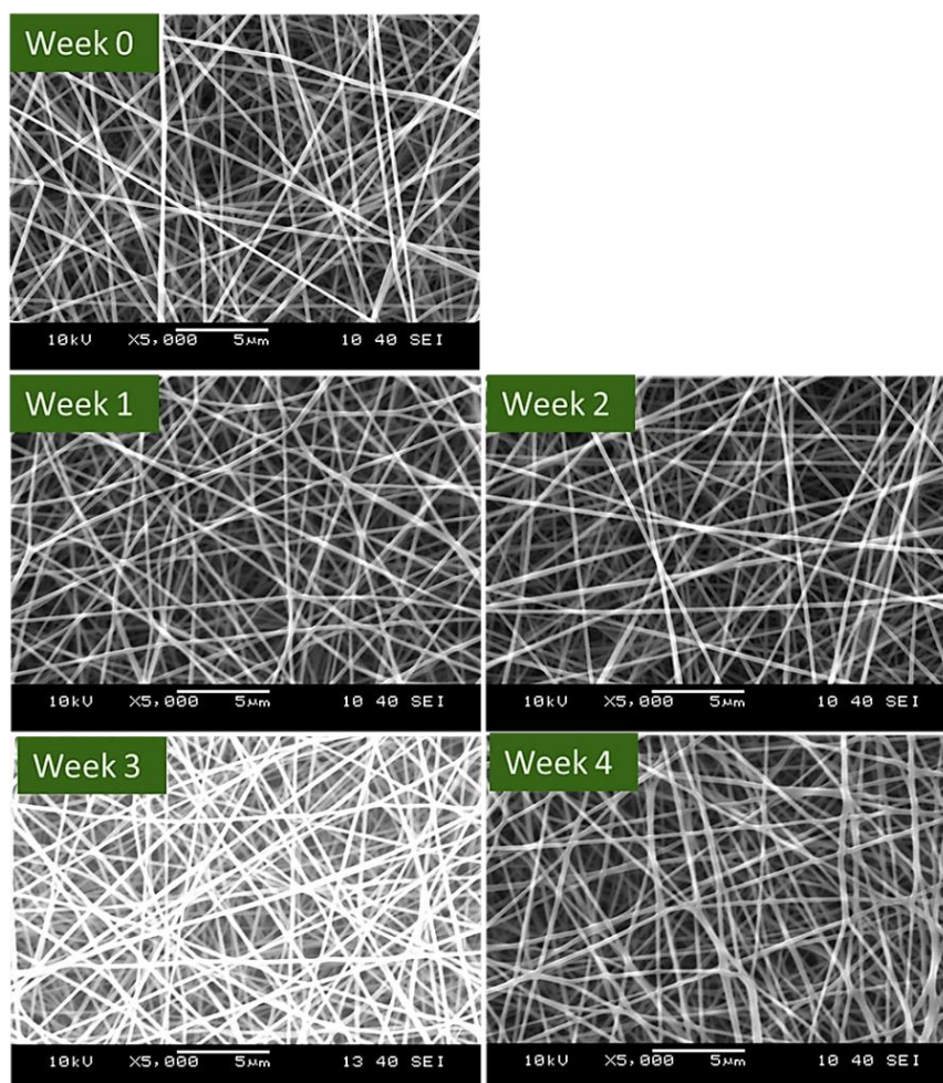
Figure 21. Scanning electron microscopic (SEM) images of the Nepafenac-loaded (NEPA-loaded) fibers at 0, 1-, 2-, 3-, and 4- weeks storage under stress conditions ( 40 \pm 2^\circ\text{C} , 75 \pm 5\% relative humidity (RH)). (magnification: 5000\times ). [III]
