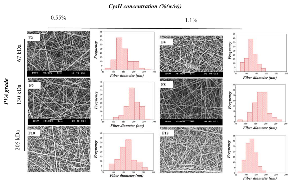
Figure 9. Scanning Electron Microscope (SEM) images and corresponding histograms of cysteamine-loaded (Cys-loaded) electrospun samples prepared from polyvinyl alcohol (PVA)/poloxamer 407 (PO-407) blends, ethylenediaminetetraacetic acid (EDTA) 0.05% (w/w), polysorbate 80 (PS-80) (0.5% (w/w)); cysteamine hydrochloride (CysH) 0.55% (w/w) (F2, F6, and F10); and CysH 1.1% (w/w) (F4, F8, and F12) (magnification: 5000 \times ). [IV]
