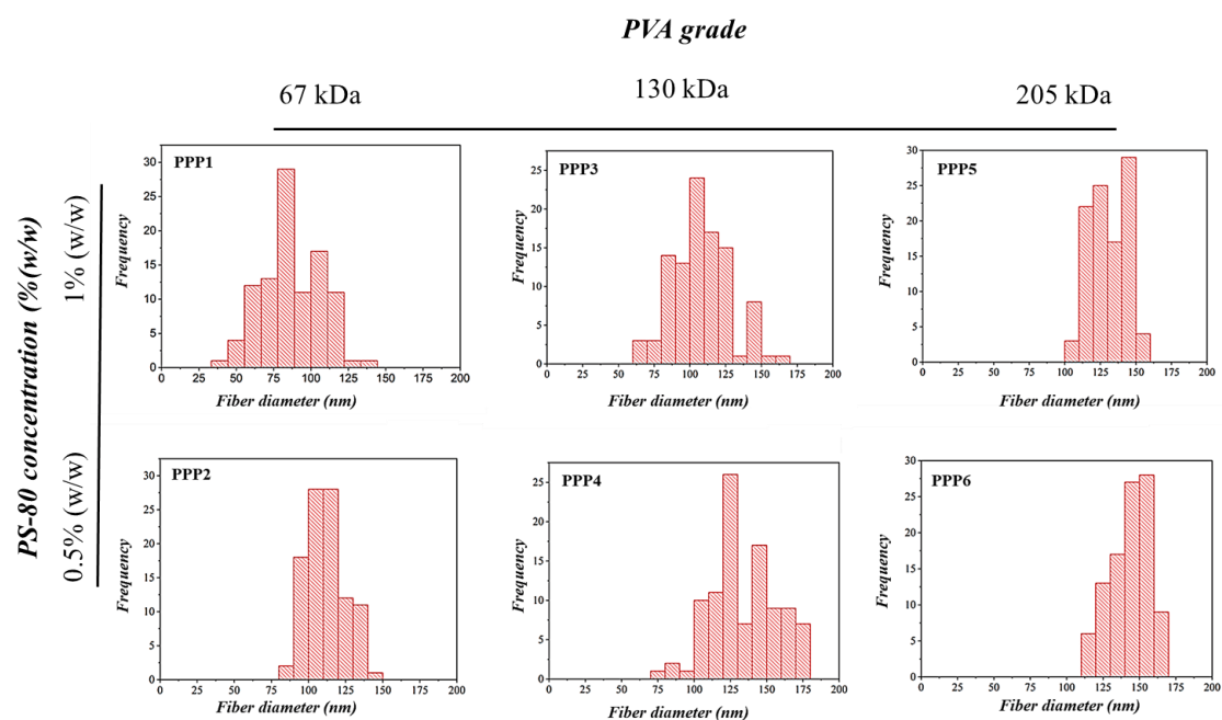
Figure 4. Fiber diameter distributions of electrospun polyvinyl alcohol (PVAs)/poloxamer 407 (PO-407)/polysorbate 80 (PS-80) samples. [IV]
