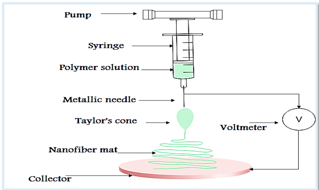
Figure 2. Schematic diagram of electrospinning process.
