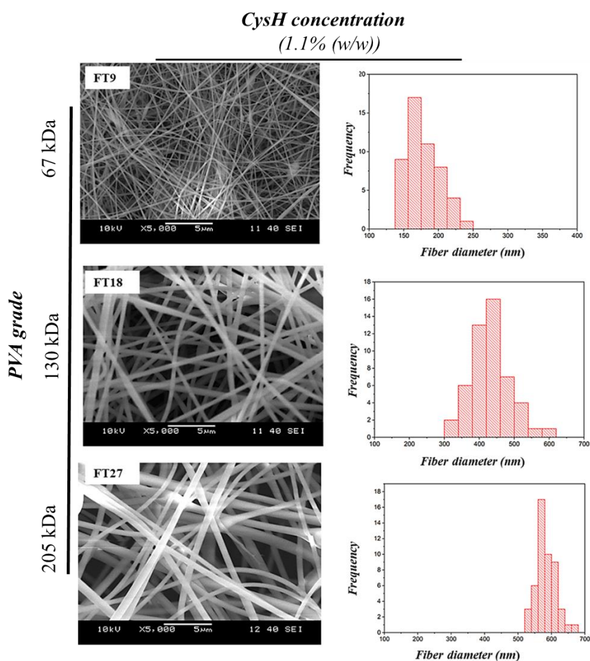
Figure 10. Scanning Electron Microscope (SEM) images and corresponding histograms of cysteamine-loaded (Cys-loaded) electrospun samples prepared from polyvinyl alcohol (PVA) / Tetraethoxysilane (TEOS) and cysteamine hydrochloride 1.1%w/w. Where FT9, FT18, and FT27 prepared from Mw~67 kDa, Mw~130 kDa, and Mw~205 kDa of PVA respectively (magnification: 5000×). [IV]
