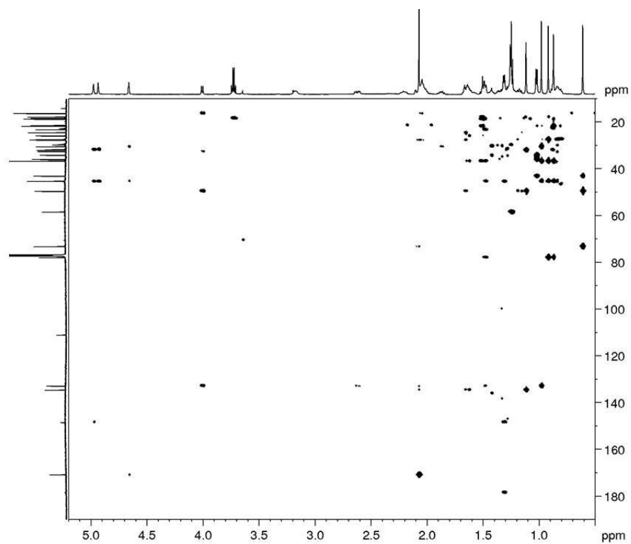
Figure A95. HMBC spectrum of BGS-11 (600 MHz, CDCl 3 , 295 K)
