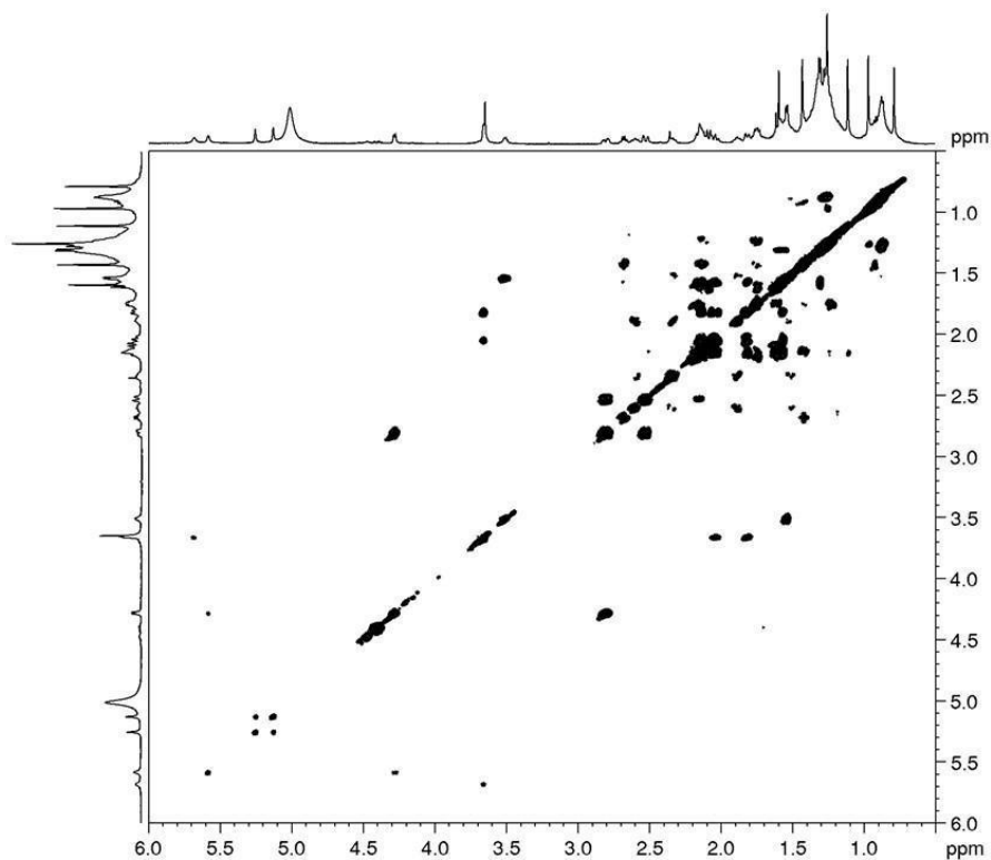
Figure A85. COSY spectrum of BGS-10 (600 MHz, \text{pyridine-}d_5 , 295 K)
