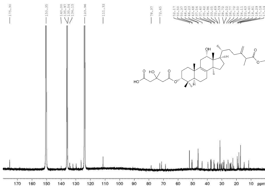
Figure A38. 13 C spectrum of BGS-5 (150 MHz, pyridine- d 5 , 295 K)
