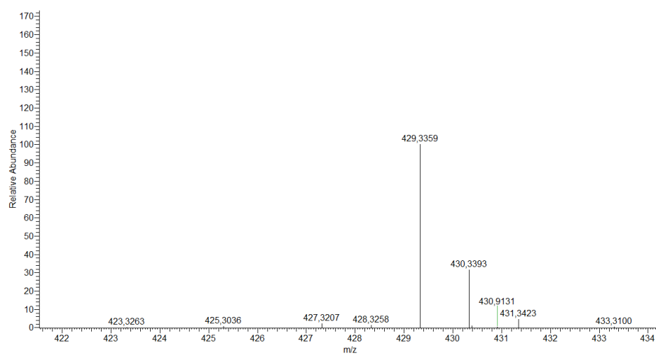
Figure A150. HRMS spectrum of XB-7
