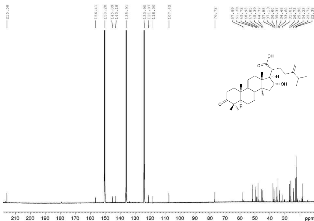
Figure A100. 13 C spectrum of BGS-12 (150 MHz, pyridine- d 5 , 295 K)
