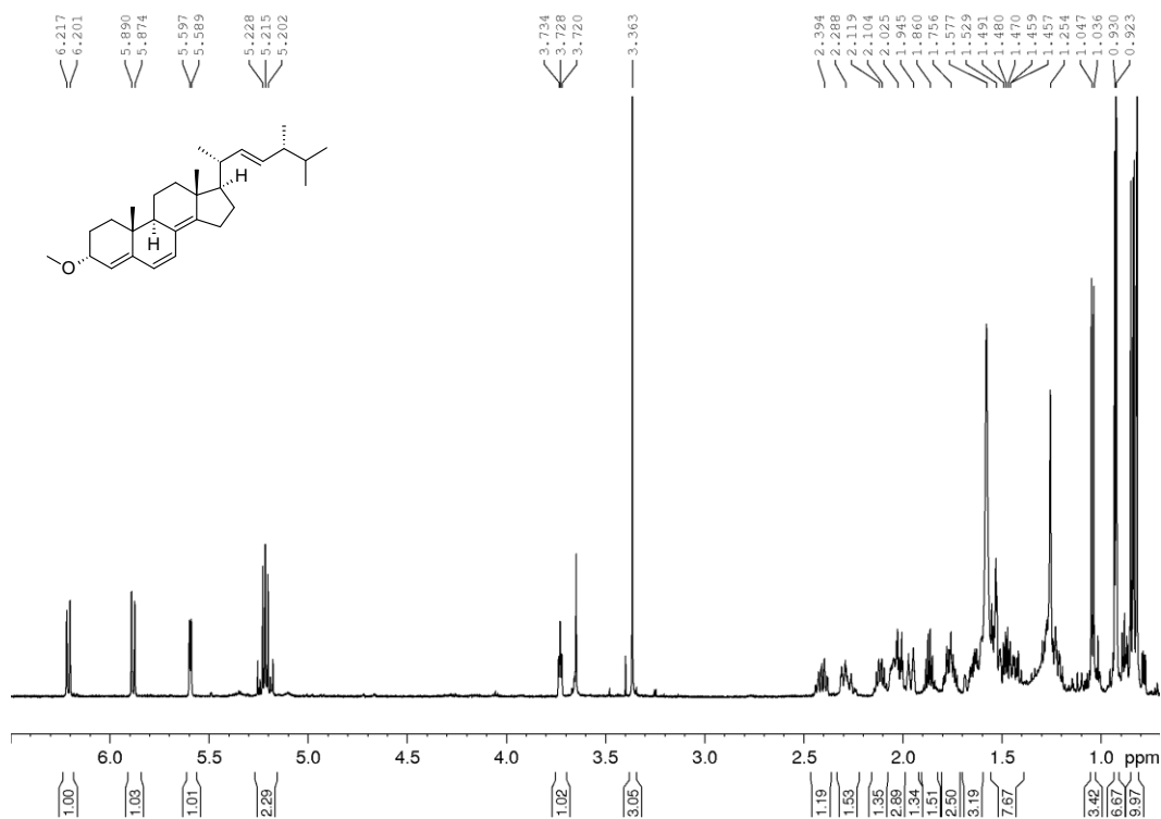
Figure A25. 1 H spectrum of XB-2 (600 MHz, CDCl 3 , 295 K)
