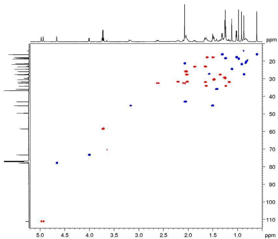
Figure A94. DEPT-edited HSQC spectrum of BGS-11 (600 MHz, CDCl 3 , 295 K)
