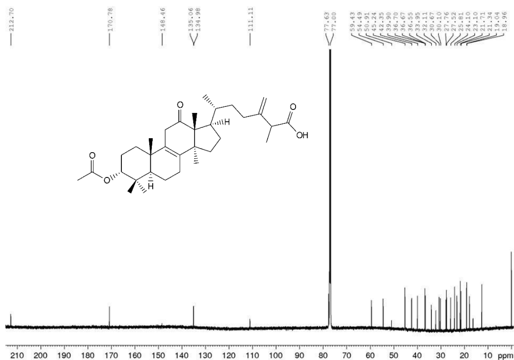
Figure A22. 13 C spectrum of BGS-3 (150 MHz, CDCl 3 , 295 K)
