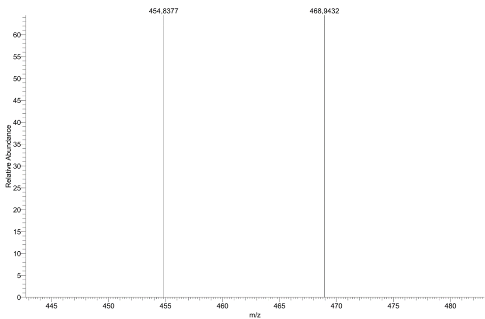
Figure A11. MS-MS spectrum of BGS-2
