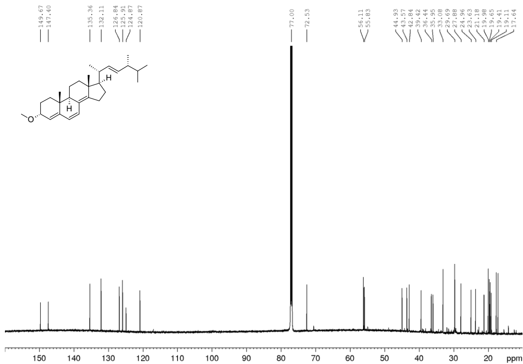
Figure A3. 13 C spectrum of XB-2 (150 MHz, CDCl 3 , 295 K)
