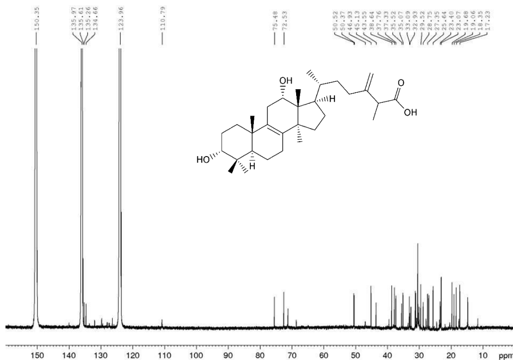
Figure A84. ^{13}\text{C} spectrum of BGS-10 (150 MHz, \text{pyridine-}d_5 , 295 K)
