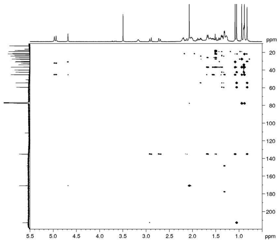
Figure A25. HMBC spectrum of BGS-3 (600 MHz, CDCl 3 , 295 K)
