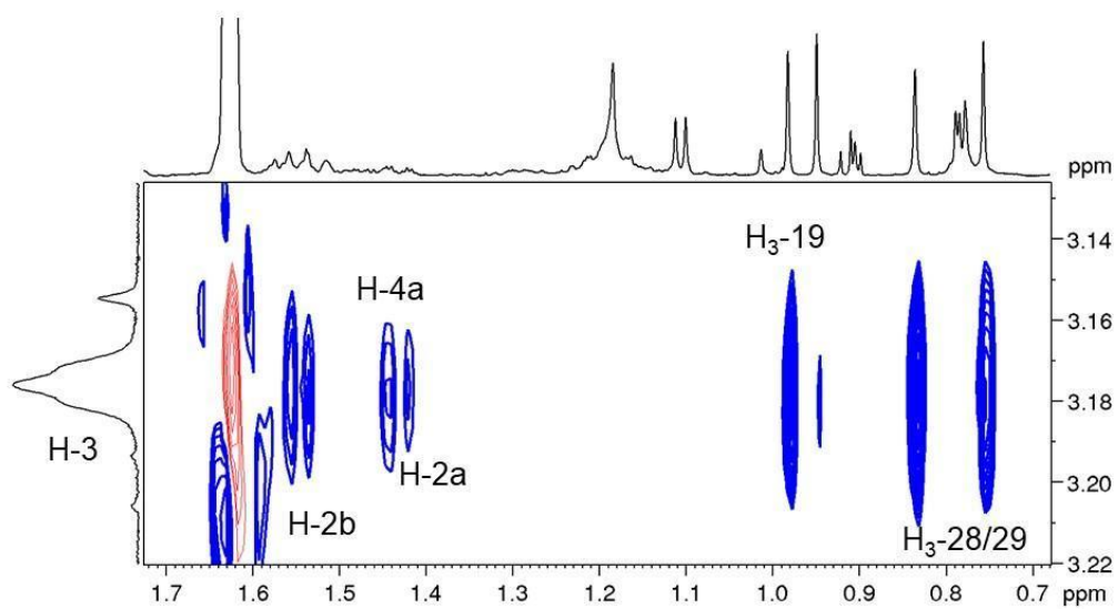
Figure A80. NOESY spectrum of BGS-9 (600 MHz, CDCl 3 , 295 K)
