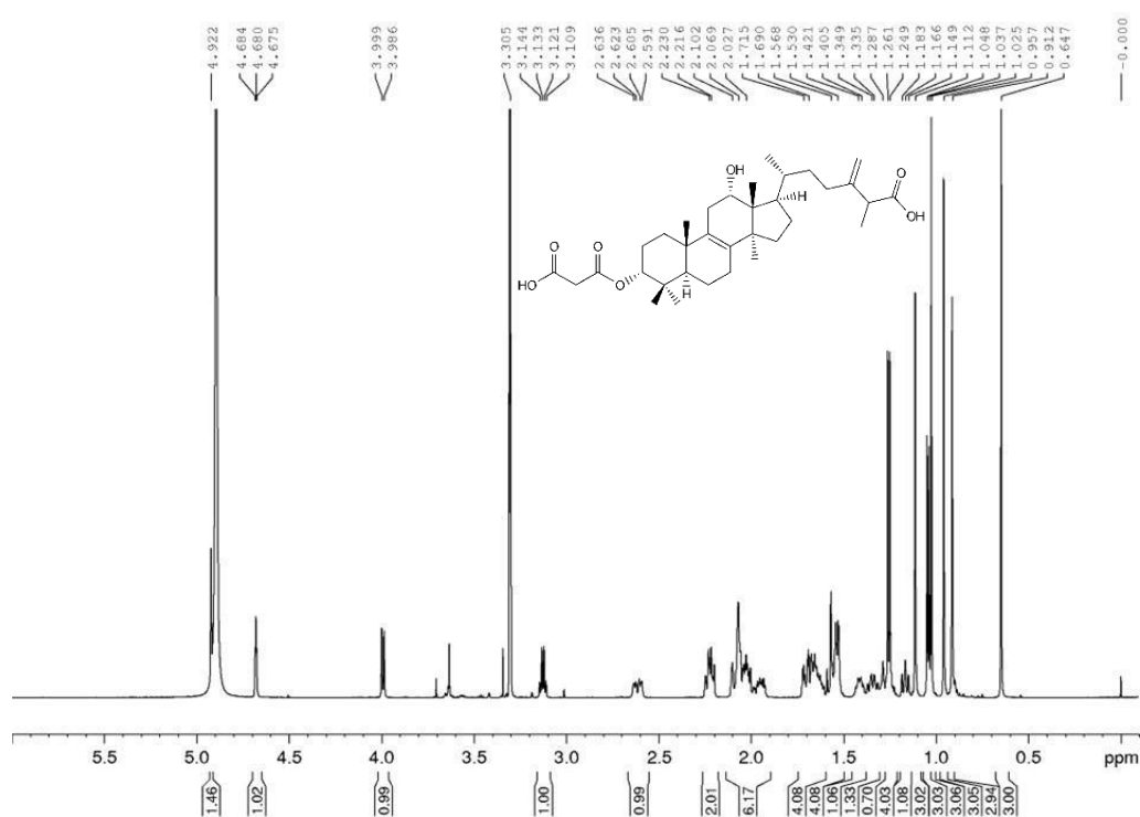
Figure A47. 1 H spectrum of BGS-6 (150 MHz, CD 3 OD, 295 K)
