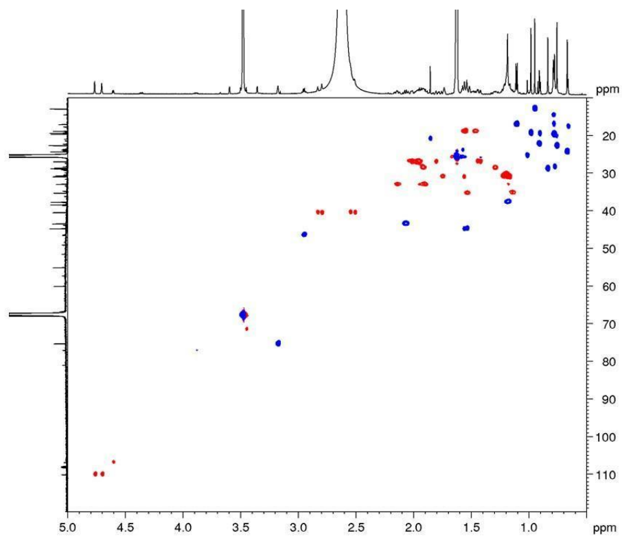
Figure A77. DEPT-edited HSQC spectrum of BGS-9 (600 MHz, CDCl 3 , 295 K)
