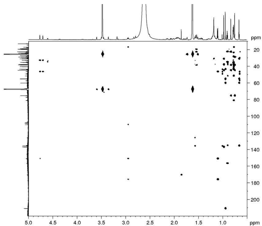
Figure A78. HMBC spectrum of BGS-9 (600 MHz, CDCl 3 , 295 K)
