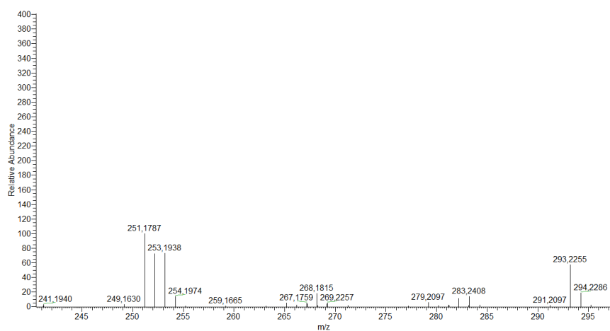
Figure A106. MS-MS spectrum of XB-1
