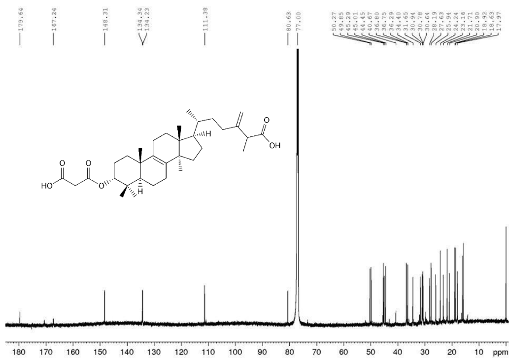
Figure A30. 13 C spectrum of BGS-4 (150 MHz, CDCl 3 , 295 K)
