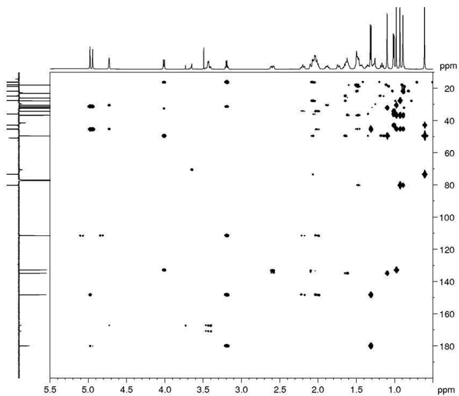
Figure A55. HMBC spectrum of BGS-6 (600 MHz, CDCl 3 , 295 K)
