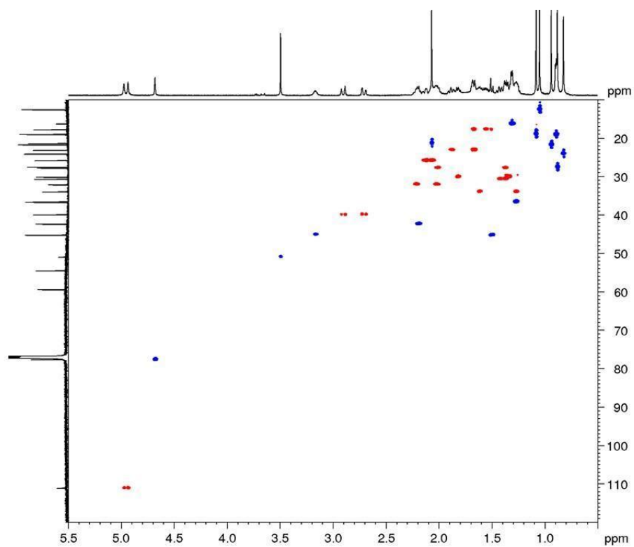
Figure A24. DEPT-edited HSQC spectrum of BGS-3 (600 MHz, CDCl 3 , 295 K)
