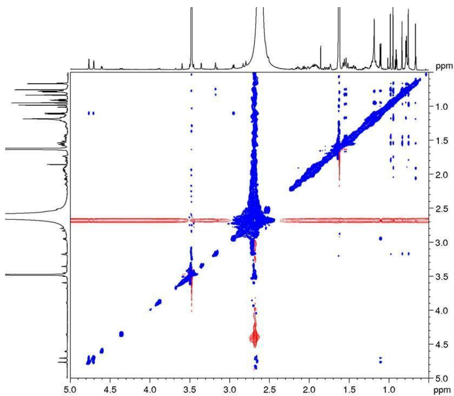
Figure A79. NOESY spectrum of BGS-9 (600 MHz, CDCl 3 , 295 K)
