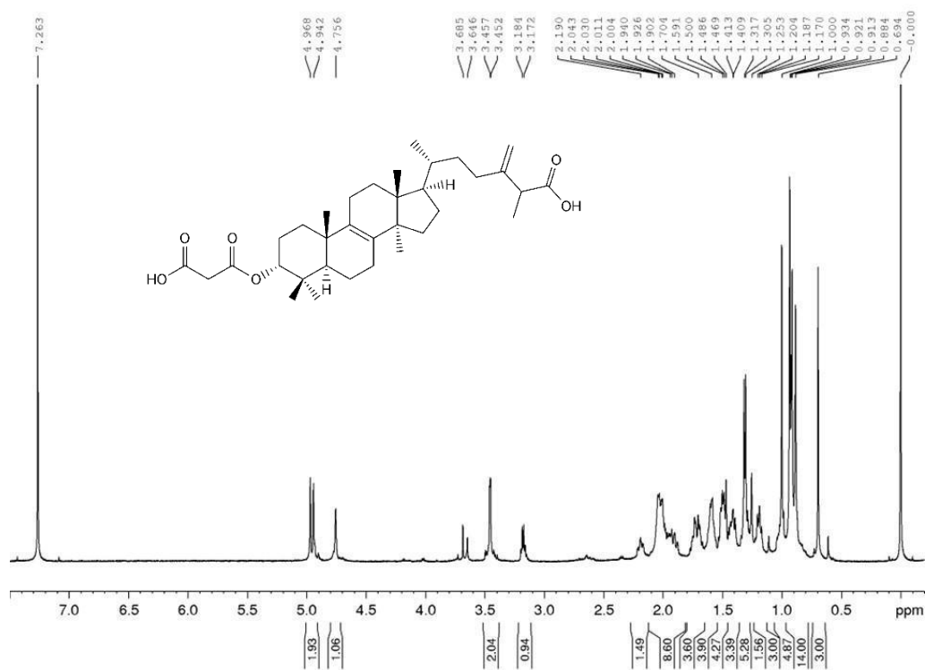
Figure A29. 1 H spectrum of BGS-4 (600 MHz, CDCl 3 , 295 K)
