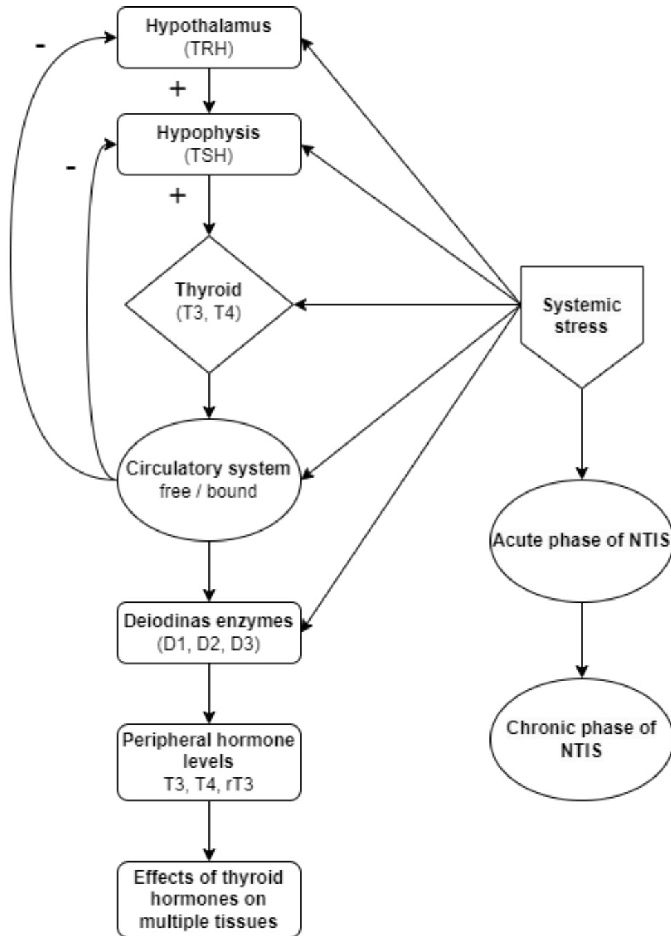
Figure 1. The hypothalamic–pituitary–thyroid axis. D1: type 1 deiodinase, D2: type 2 deiodinase, D3: type 3 deiodinase, NTIS: non-thyroidal illness syndrome, rT3: reverse T3, TRH: thyrotropin-releasing hormone, TSH: thyroid stimulating hormone, T3: triiodothyronin, T4: thyroxine
