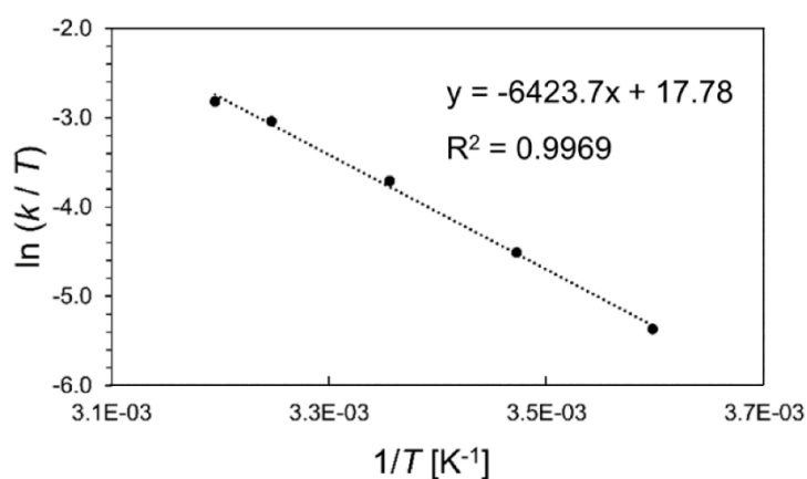
Figure 33. Eyring-plot of the k_{ex} values from the average values of H3' and H5' volume integrals (75).
