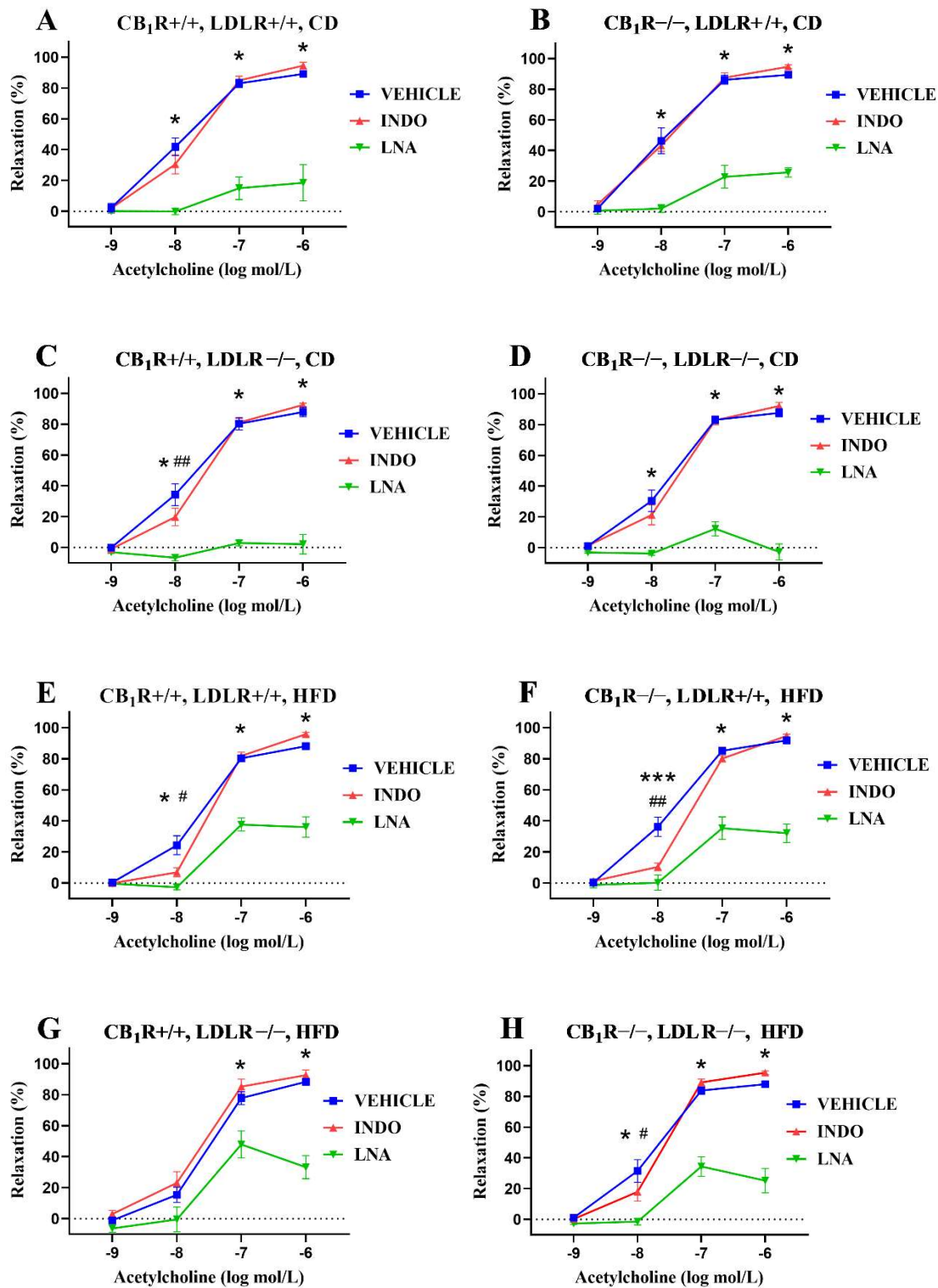
Figure 6. Effects of specific inhibitors of endothelial nitric oxide synthase N \omega -nitro-L-arginine and of cyclooxygenase indomethacin on vasodilatory responses in aortas of CB_1R and LDLR wild-type and -knockout mice kept on control diet and high-fat diet. Panel (A). Effects of specific inhibitors on vasodilation in CB_1R^{+/+}, LDLR^{+/+} , control diet group (n=5-6). Panel (B). Effects
