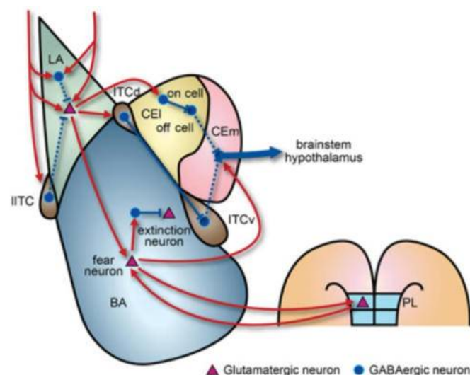
Figure 6. Successful fear conditioning involves the interplay of glutamatergic and GABAergic neurons in the BLA. During fear conditioning, incoming information
