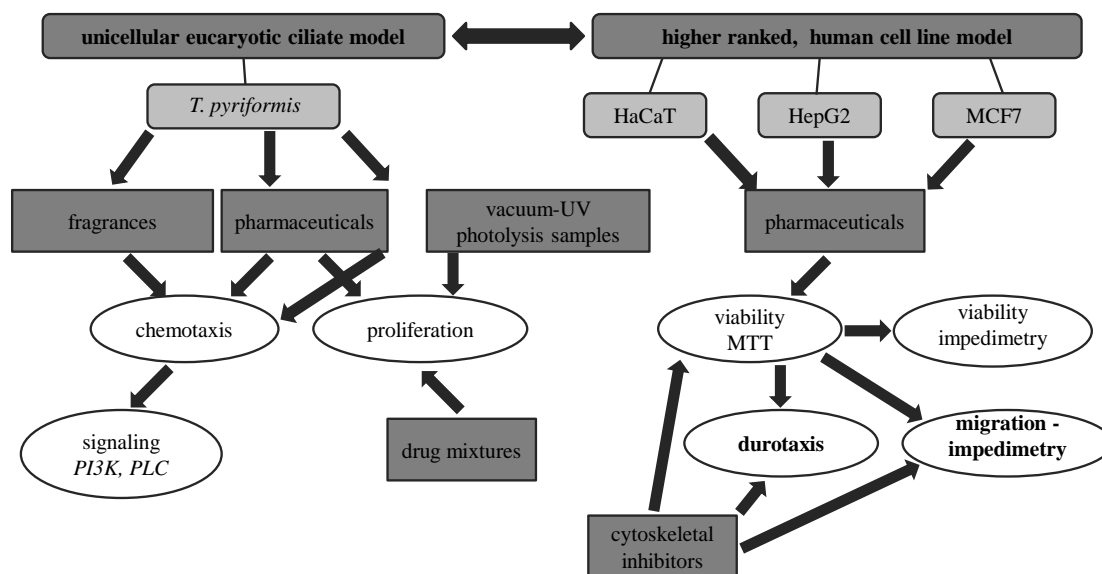
Fig. 1: Overview of the applied model systems and most important biological assays
