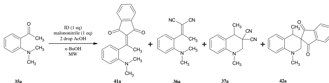
Figure 52: Competition experiment with malononitrile and ID
