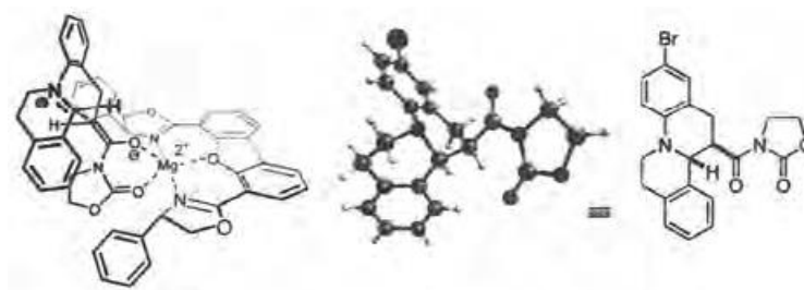
Figure 34: Proposed transition-state leading to major diastereomer. Absolute configuration of brominated compound (X-ray)
