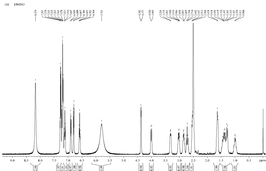
1 H NMR spectrum of [cis-cis-(±)-6-Phenyl-1H-2,3,4,4a,5,6-hexahydropyrido[1,2-a]quinolin-5-yl]methanamine dihydrochloride ( 40f cis-cis ); 400 MHz.
