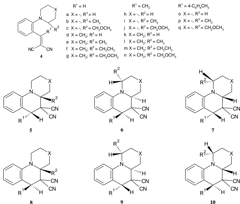
Figure 9: Vinyl compounds with various \text{R}^1 and \text{R}^2 substituents and their cyclized products
