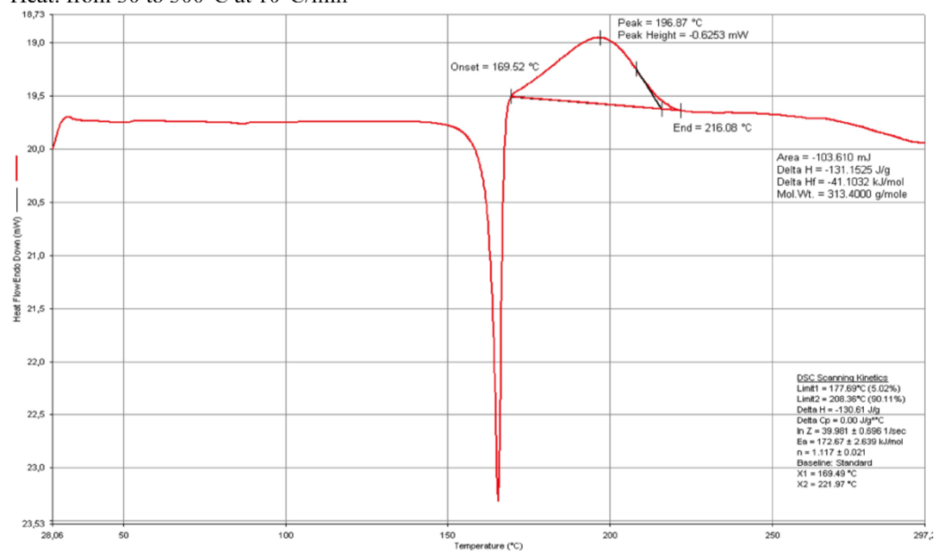
Figure 46: DSC curves of compounds 36e (upside) and 36f (bottomside)
