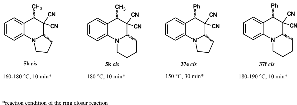
Figure 47: The heating test of the pure cis isomers
