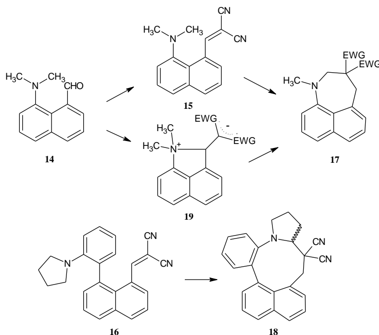
Figure 20: Formation of benzo[ c,d ]indolium ( 19 ), azepine ( 17 ) and azonine ( 18 ) ring systems
