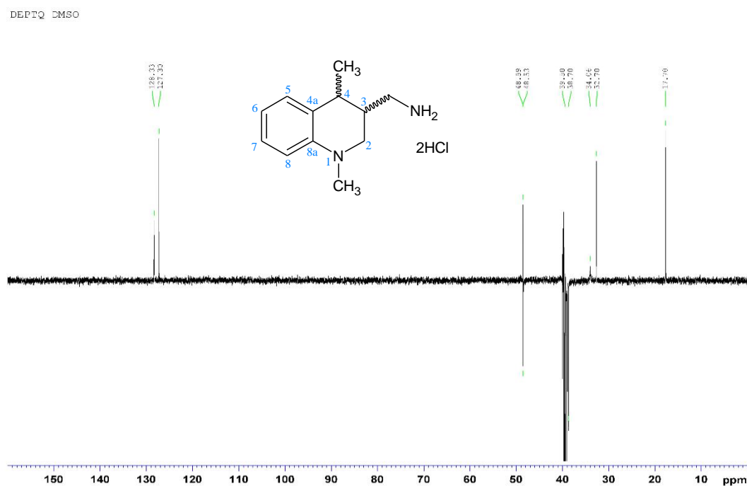
DEPTQ spectrum of ( cis -( \pm )-1,4-Dimethyl-1,2,3,4-tetrahydroquinolin-3-yl)methanamine dihydrochloride ( 40a cis ); 125 MHz.
