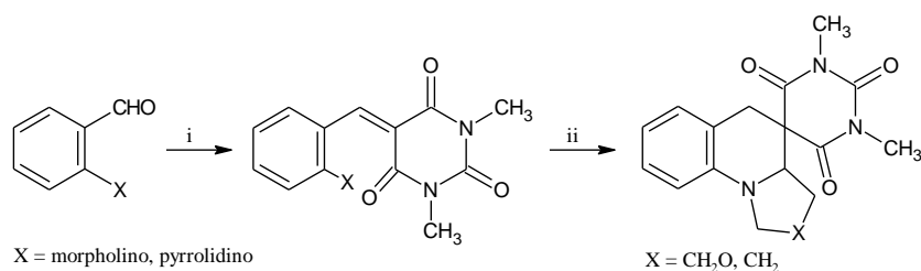
Figure 27: Reagents and conditions: i) DMB, EtOH, r.t., 15 min for morpholine derivative, 10 min for pyrrolidine derivative; ii) toluene, AlCl 3 , 70 °C, 3 h for morpholine derivative, the vinyl compound substituted with pyrrolidino group could not be isolated in pure form since ring closed product was also formed.
