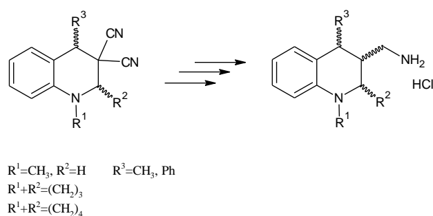
Figure 43: Synthesis of potential SSAO active aminomethyl derivatives
