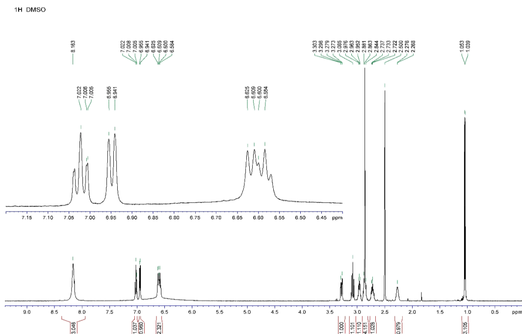
^1\text{H} NMR spectrum of ( cis -( \pm )-1,4-Dimethyl-1,2,3,4-tetrahydroquinolin-3-yl)methanamine dihydrochloride ( 40a cis ); 500 MHz.
