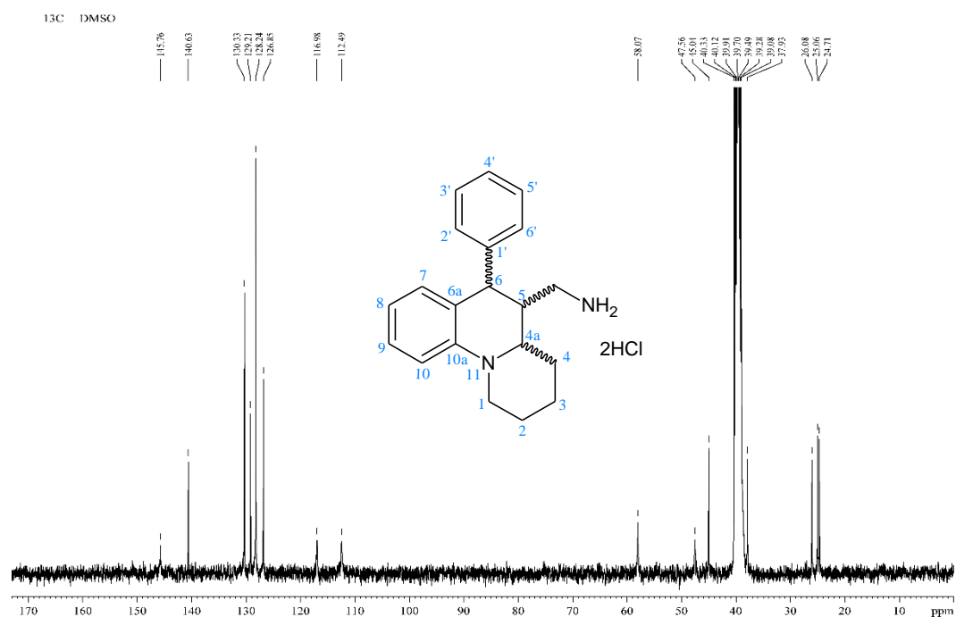
13 C NMR spectrum of [cis-cis-(±)-6-Phenyl-1H-2,3,4,4a,5,6-hexahydropyrido[1,2-a]quinolin-5-yl]methanamine dihydrochloride ( 40f cis-cis ); 100 MHz.
