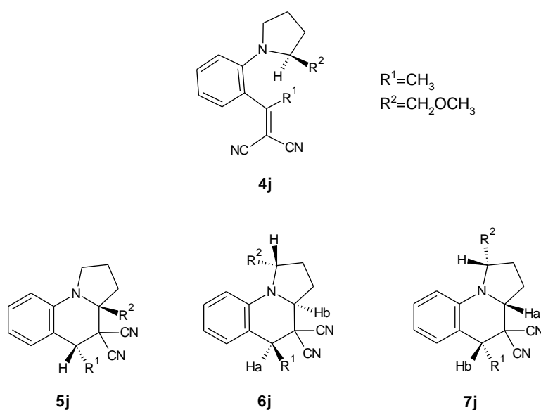
Figure 13: Chiral vinyl compound with S configuration and its ring closed products
