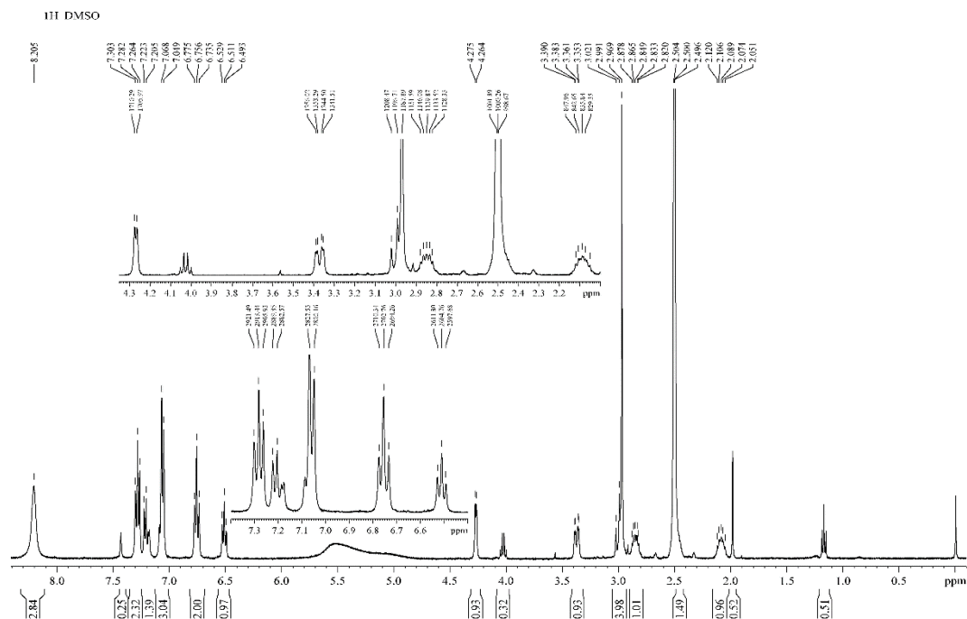
^1\text{H} NMR spectrum of [ cis -(±)-1-Methyl-4-phenyl-1,2,3,4-tetrahydroquinolin-3-yl]methanamine dihydrochloride ( 40d cis ); 400 MHz.
