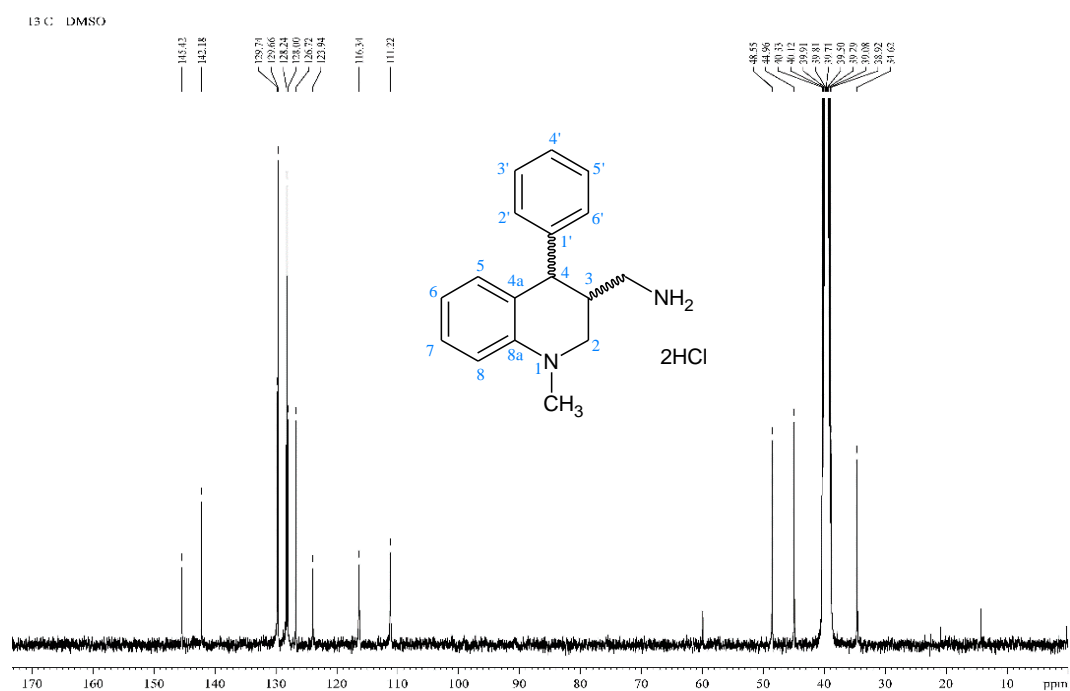
^{13}\text{C} NMR spectrum of [ cis -(±)-1-Methyl-4-phenyl-1,2,3,4-tetrahydroquinolin-3-yl]methanamine dihydrochloride ( 40d cis ); 100 MHz.
