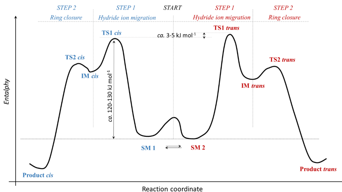
Figure 55. Schematic illustration of enthalpy profile of the reaction mechanism.
