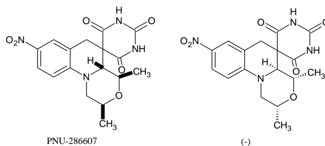
Figure 28: Structure of PNU-286607 (±) and its active enantiomer (-)
