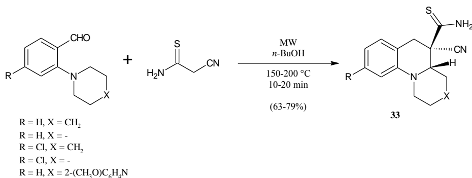
Figure 31: Microwave-assisted synthesis of fused 3-thiocarbamoylquinolines ( 33 ) via the tert -amino effect
