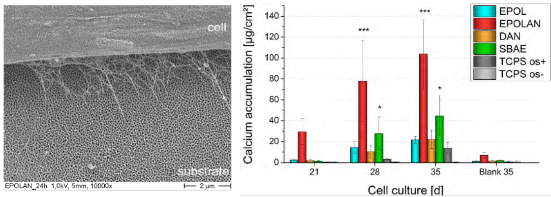
Figure 18. Adherence and osteogenic differentiation of MSC on titanium-oxide nanotubular array. The SEM image shows that MSCs adhere to the nanosurface through nanotubular projections of the ECM. The bar diagram shows significantly higher mineralization on nanotubular array (induced by soluble cues) than on other nano-, and micro-rough surfaces. EPOL: electromechanically polished (featureless) surface; EPOLAN: nanotubular array; DAN: nanopitted surface; SBAE: sand-blasted/acid etched microrough surface; TCPS: tissue culture polystyrene (internal reference) 208 .
