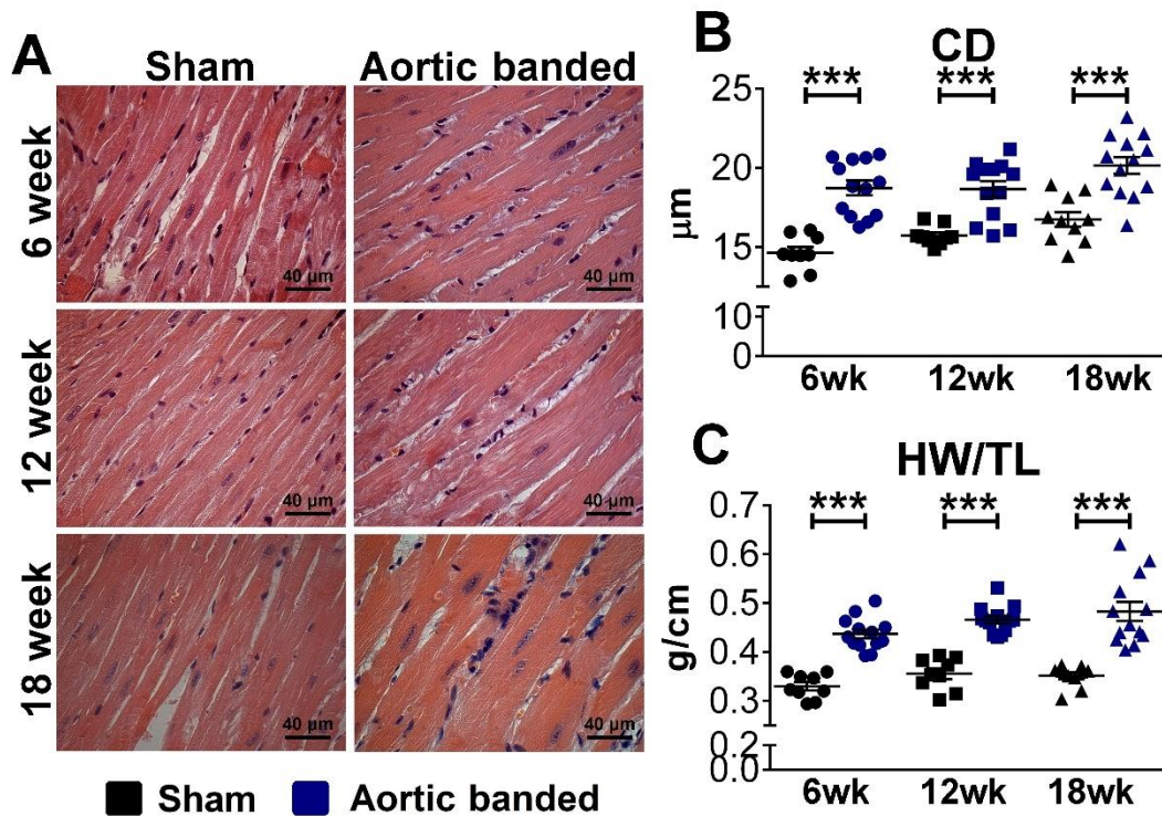
Figure 9. Macroscopic and microscopic myocardial hypertrophy markers. Representative photomicrographs (A) of hematoxylin and eosin staining (magnification 200x, scale bar: 40 \mu\text{m} ) are shown demonstrating enlarged cardiomyocytes in the aortic banded groups. Cardiomyocyte diameter (CD) (B) and heart weight-to-tibial length (HW/TL) (C) increased in the aortic banded groups at week 6, 12 and 18 compared to sham groups. ***: P<0.001 vs. corresponding sham.
