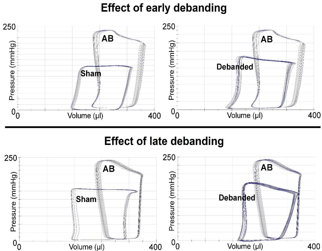
Figure 27. Representative left ventricular (LV) pressure-volume (P-V) steady-state loops demonstrating the effect of early and late debanding on left ventricular function. In the aortic banded (AB) groups at week 12 and 18, the width of the loops was substantially smaller compared to the corresponding age-matched sham groups, suggesting impaired LV systolic function. Both early and late debanding effectively increased the width of the P-V loops, indicating that pressure unloading therapy performed either at early or late time points successfully improved LV systolic performance.
