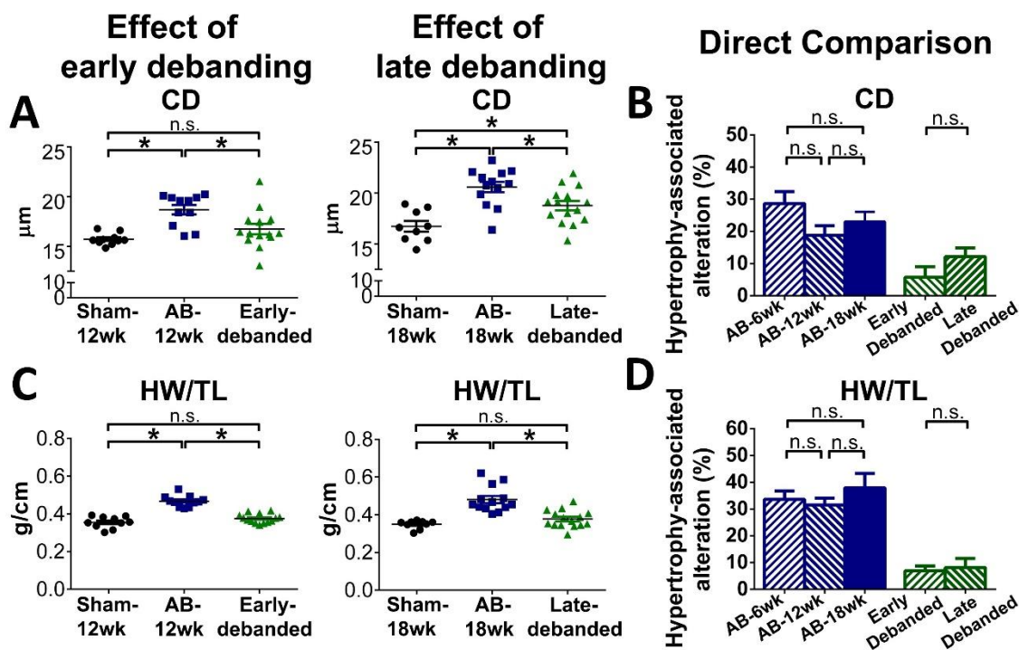
Figure 20. Effect of early and late debanding on macroscopic and microscopic myocardial hypertrophy markers.: Cardiomyocyte diameter (CD) and heart weight-to-tibial length ratio (HW/TL) were increased in the aortic banded (AB) groups at week 12 and 18 compared to their age-matched sham groups. Both early and late debanding resulted in substantial decrement of CD and HW/TL ( A, C ). No differences could be observed in the extent of CD and HW/TL regression between the early and the late debanded groups ( B, D ). *: P < 0.05 .
