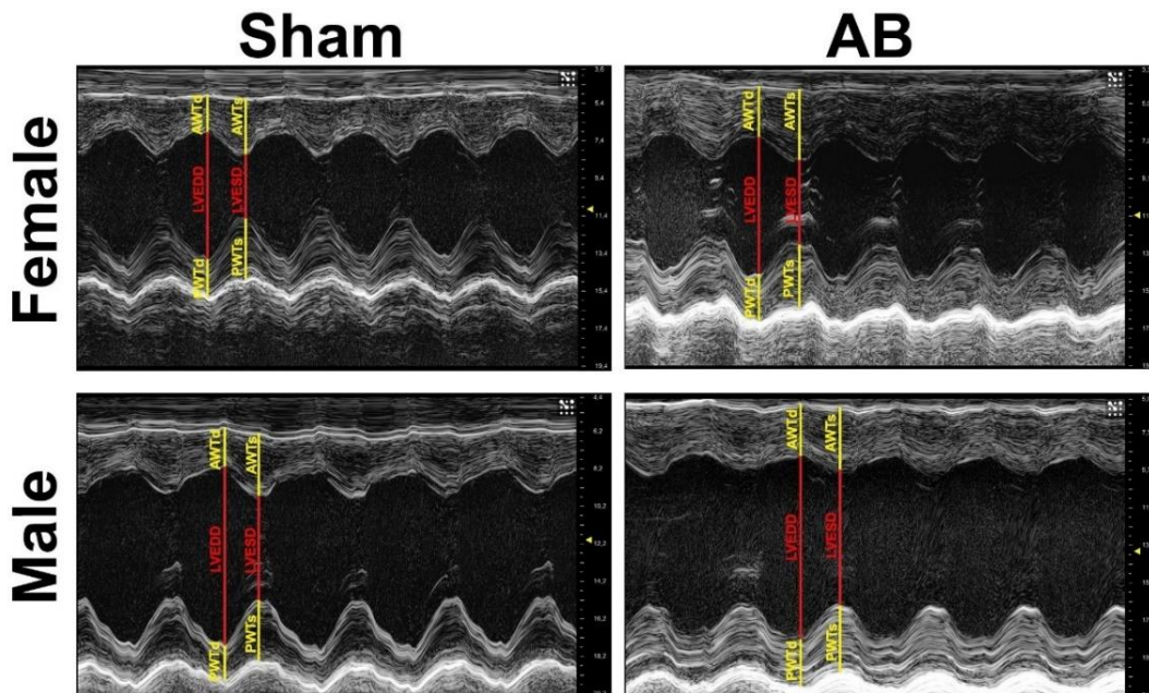
Figure 32. Representative echocardiographic recordings demonstrating sex-related differences in male and female aortic banded (AB) rats at week 12. The female AB was associated with increased left ventricular (LV) wall thicknesses, concentric geometry and maintained systolic function. In contrast the male AB was characterized by increased LV wall thicknesses, eccentric remodeling and decreased systolic function. AWT indicates anterior wall thickness, PWT: posterior wall thickness, LVEDD: left ventricular end-diastolic diameter, LVESD: left ventricular end-systolic diameter, s: systole, d: diastole.
