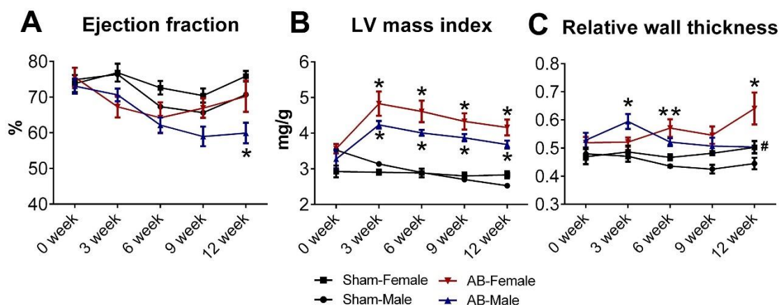
Figure 33. Echocardiographic follow-up during the development of pressure overload-induced myocardial hypertrophy in male and female rats. The female aortic banded (AB) group was associated with maintained ejection fraction (A), enhanced left ventricular (LV) mass index (B) and increased relative wall thickness (C) at both early (week 6) and later time points (week 12). The male AB group was also characterized by preserved ejection fraction (A), increased LV mass index (B) and increased relative wall thickness (C) at a relatively early time point (week 6). However, deterioration of ejection fraction (A) and decrement of relative wall thickness (B) took place in male AB rats at week 12, leading to substantial differences between the two sexes. *P < 0.05 vs. age and sex-matched sham. #: P < 0.05 vs. female AB.
