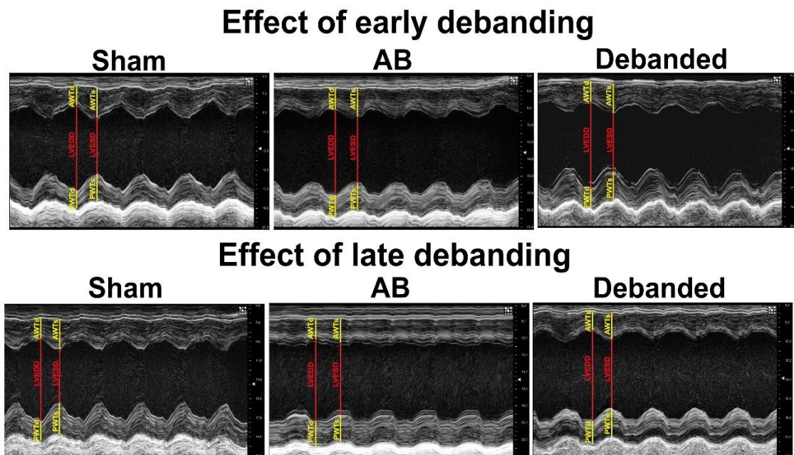
Figure 17. Representative echocardiographic images during the development of pressure overload-induced left ventricular myocardial hypertrophy and its regression after early and late debanding. Characteristic M-mode echocardiographic recordings at the midpapillary muscle level are shown at week 12 (in case of early debanding) and at week 18 (in case of late debanding) in the sham, the aortic banded (AB) and the debanded groups. Myocardial hypertrophy effectively regressed after early and late debanding as well. AWT: anterior wall thickness, PWT: posterior wall thickness, LVEDD: left ventricular (LV) end-diastolic diameter, LVEDS: LV end-systolic diameter, s: systole, d: diastole.
