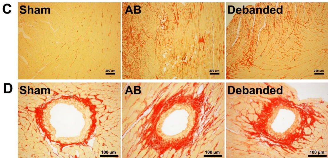
Figure 24. Representative histological photomicrographs of interstitial and perivascular fibrosis demonstrating regression of reactive fibrosis in the early debanded group and persisting collagen accumulation in the late debanded group. Representative photomicrographs of picrosirius red staining are shown demonstrating interstitial fibrosis (A, C) (magnification 50x, scale bar: 200μm) and perivascular fibrosis (B, D) (magnification 100x, scale bar: 100μm). AB: aortic banding.
