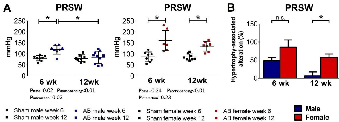
Figure 40. Alterations in preload recruitable stroke work (PRSW) in male and female aortic banded (AB) rats. PRSW was enhanced in both male and female AB rats at week 6 (A) compared to their corresponding sham groups. Female AB rats demonstrated increased PRSW at week 12 as well. In contrast, the augmented LV contractility (increased PRSW) reduced to the control's level in male AB rats at week 12 (A). Accordingly, robust differences were observed in PRSW between the two sexes at week 12 (B). *: P<0.05 .
