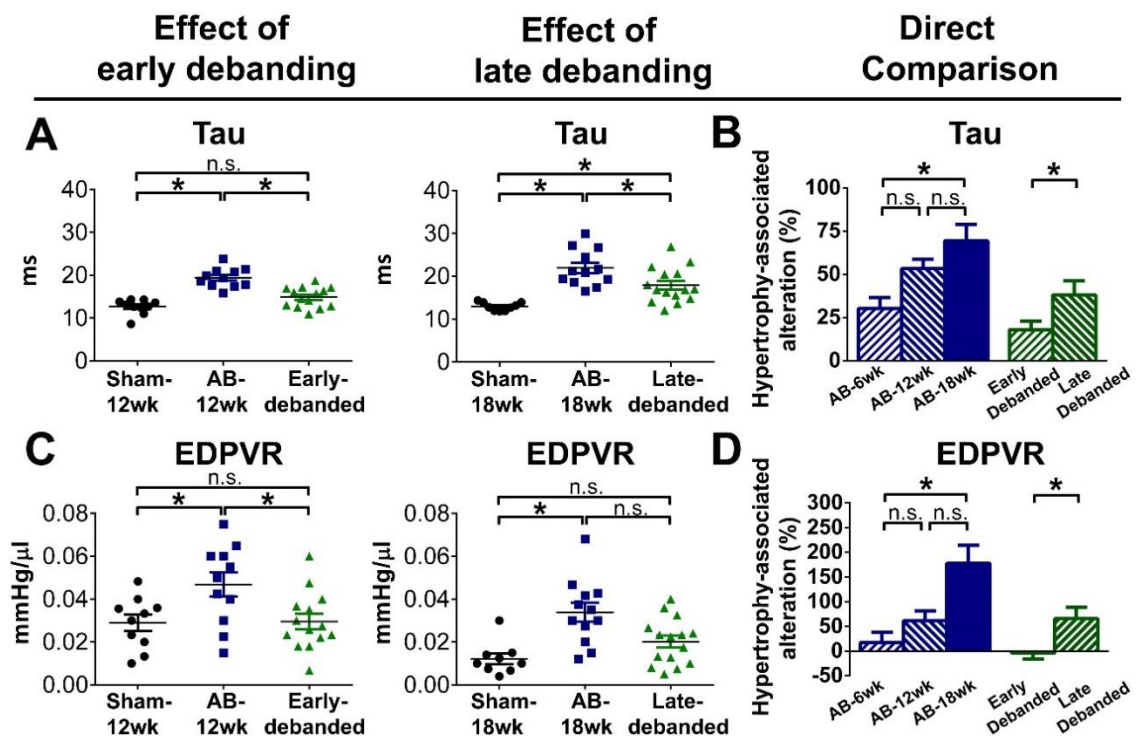
Figure 31. Diastolic function during the development of aortic banding (AB)-induced LVH and its regression by early and late debanding. Prolongation of the active relaxation time constant (Tau) and increased myocardial stiffness (assessed by the elevated slope of the end-diastolic pressure-volume relationship [EDPVR]) were detected in the AB groups at week 12 and 18 ( A, C ). Debanding the aortic constriction at an early time point effectively improved both aspects of diastolic function ( A, C ). In contrast, late debanding failed to normalize diastolic dysfunction. Accordingly, robust differences were observed between the early and the late debanding groups ( B, D ). *: P < 0.05 .
