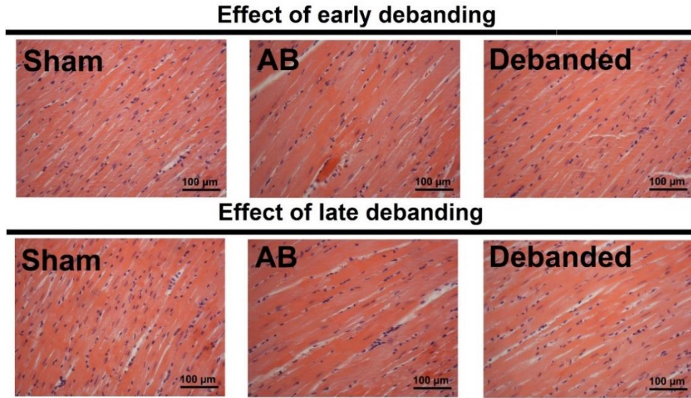
Figure 21. Representative microphotographs demonstrating enlargement of cardiomyocytes in the aortic banded (AB) groups and their regression in both the early and late debanded groups: Hematoxylin and eosin (magnification 200x, scale bar: 100 \mu m) stained sections are shown. AB indicates aortic banding.
