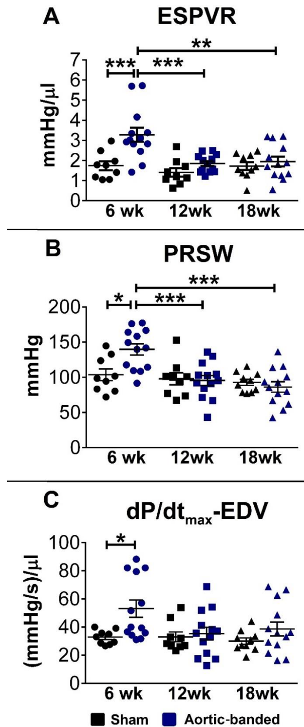
Figure 16. Left ventricular contractility parameters during the development and progression of pressure overload-induced left ventricular myocardial hypertrophy. Both the slope of the end-systolic pressure-volume relationship (ESPVR) (A), preload recruitable stroke work (PRSW) (B) and the slope of the maximal systolic pressure increment ( dP/dt_{max} )-end diastolic volume (EDV) relationship (C) were increased in the aortic banded (AB) group at week 6 compared to the corresponding sham group, suggesting enhanced left ventricular contractility. This contractility augmentation diminished in the AB groups at week 12 and 18. *: P < 0.05 . **: P < 0.01 . ***: P < 0.001 .
