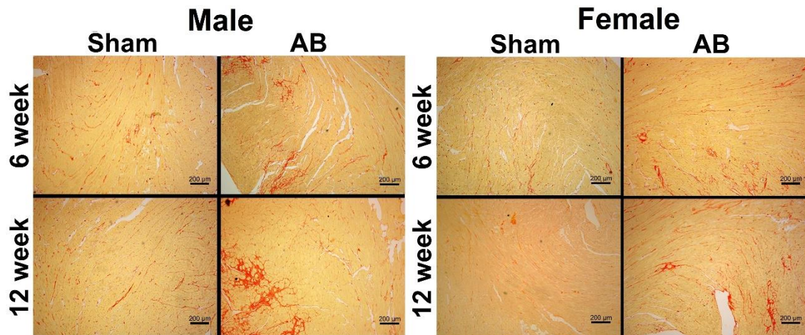
Figure 37. Representative histological photomicrographs demonstrating enhanced interstitial fibrosis in male and female aortic banded (AB) rats. Picosirius red-stained sections (magnification 50x, scale bar: 200 µm) are shown. Collagen accumulation (indicated by the red area) was observed in both male and female AB rats at week 6. Furthermore, fibrosis was progressed to a greater extent in male but not in female AB rats at week 12.
