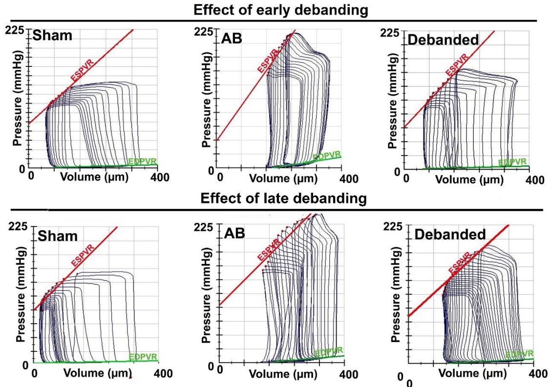
Figure 28. Representative pressure volume loops demonstrating characteristic alterations in the aortic banded (AB) groups and in the early and late debanded groups. Original recordings were obtained at different preloads during transient vena cava occlusion. The slope of end-systolic pressure volume relationship (ESPVR) did not differ among the study groups. In contrast, the slope of the end-diastolic pressure volume relationship (EDPVR) was increased in the AB groups, suggesting impaired myocardial stiffness. Increased EDPVR was normalized in the early debanded group, while it persisted in the late debanded group.
