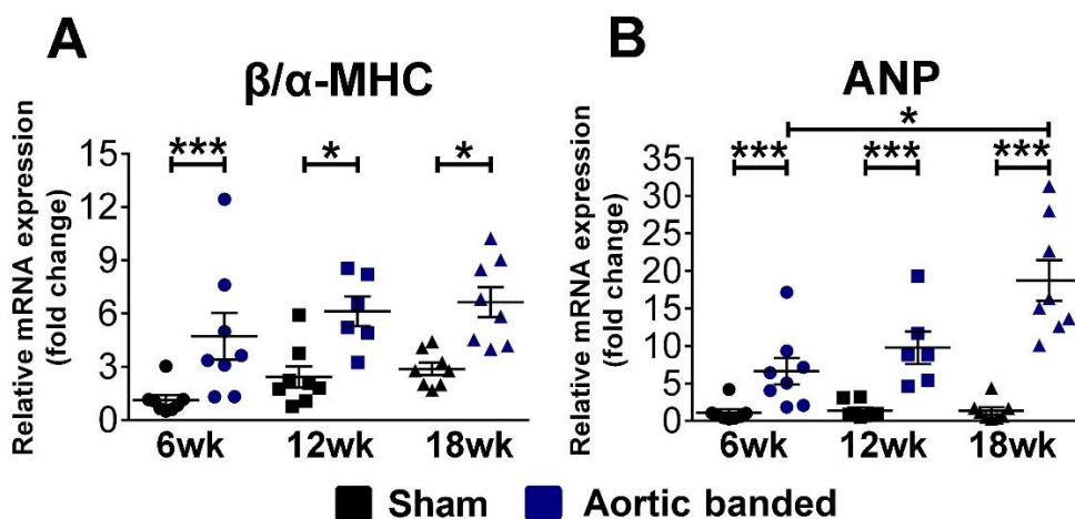
Figure 10. Fetal gene expression during pressure overload-induced myocardial hypertrophy. mRNA expression of beta-to-alpha myosin heavy chain ( \beta/\alpha\text{-MHC} ) (A) and atrial natriuretic peptide (ANP) (B) increased in the aortic banded groups at week 6, 12 and 18 compared to the age-matched sham groups. *: P<0.05 vs. age-matched sham. ***: P<0.001 vs. age-matched sham.
