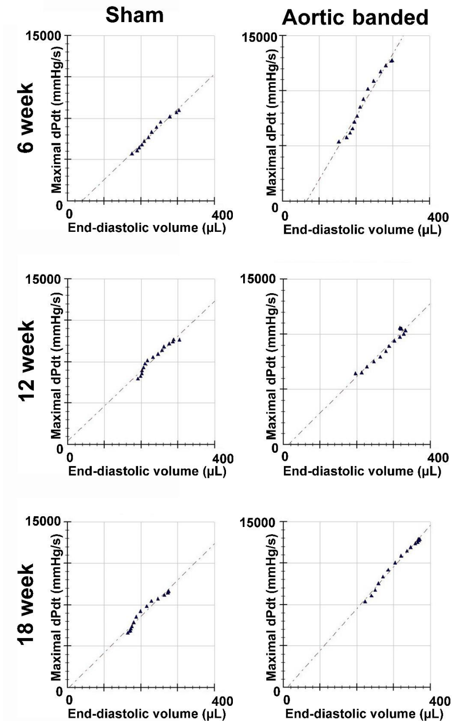
Figure 15. Alterations in the slope of the maximal systolic pressure increment ( dP/dt_{max} )-end diastolic volume (EDV) relationship during the progression of pressure overload-induced myocardial hypertrophy. dP/dt_{max} -EDV indicated augmented left ventricular (LV) contractility in the aortic banded (AB) group at week 6 compared to the corresponding sham group. The contractility enhancement diminished in the AB groups at week 12 and 18.
