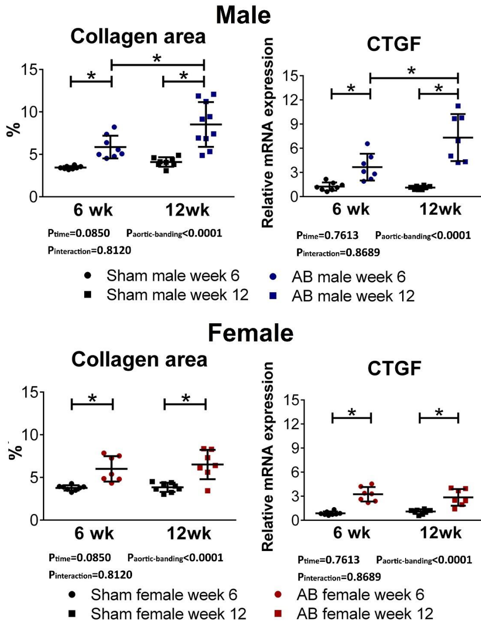
Figure 35. The effect of sex on fibrosis markers. Collagen area and mRNA level of connective tissue growth factor (CTGF) were increased in male and female aortic banded (AB) rats at week 6 and 12 as well when compared to their age-matched sham groups. Furthermore, fibrosis showed significant progression from week 6 to week 12 in male AB rats, while in female AB rats the collagen area and CTGF expression was comparable at week 6 and week 12. *: P<0.05 .
