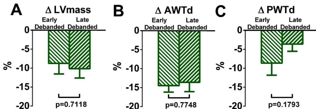
Figure 19. Direct comparison of left ventricular hypertrophy regression between the early and the late debanded groups. Left ventricular mass (LVmass) (A), anterior wall thickness in diastole (AWTd) (B) and posterior wall thickness in diastole (PWTd) (C) regressed to a similar extent in the early and the late debanding groups.
