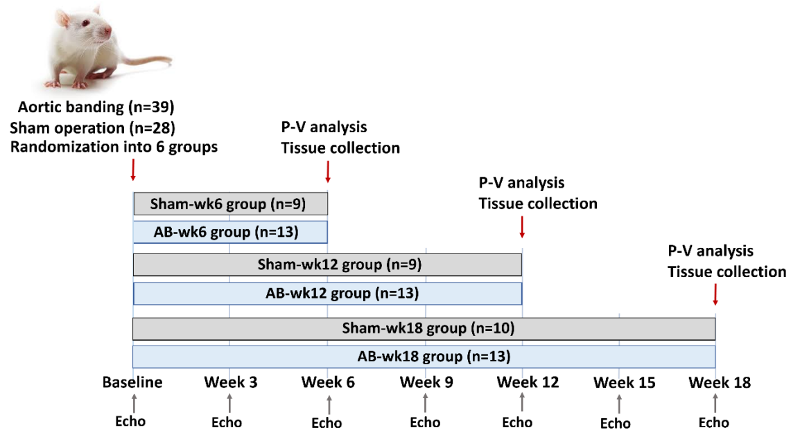
Figure 4. Schematic illustration of the experimental protocol of Study 1. At baseline, the rats underwent abdominal aortic banding ([AB]; n=39) or sham operation (n=28) and were subsequently randomized into 6 groups. In the Sham-wk6 (n=9) and AB-wk6 (n=13) groups, pressure-volume (P-V) analysis and tissue collection were performed 6 weeks after AB/sham operations. In the Sham-wk12 (n=9) and AB-wk12 (n=13) groups, P-V analysis and tissue collection were performed 12 weeks after AB/sham operations. In the Sham-wk18 (n=10) and AB-wk18 (n=13) groups, P-V analysis and tissue collection were performed 18 weeks after AB/sham operations. Furthermore, repetitive echocardiographic measurements at baseline, week 3, 6, 9, 12, 15 and 18 were also carried out in the Sham-wk18 and AB-wk18 groups.
