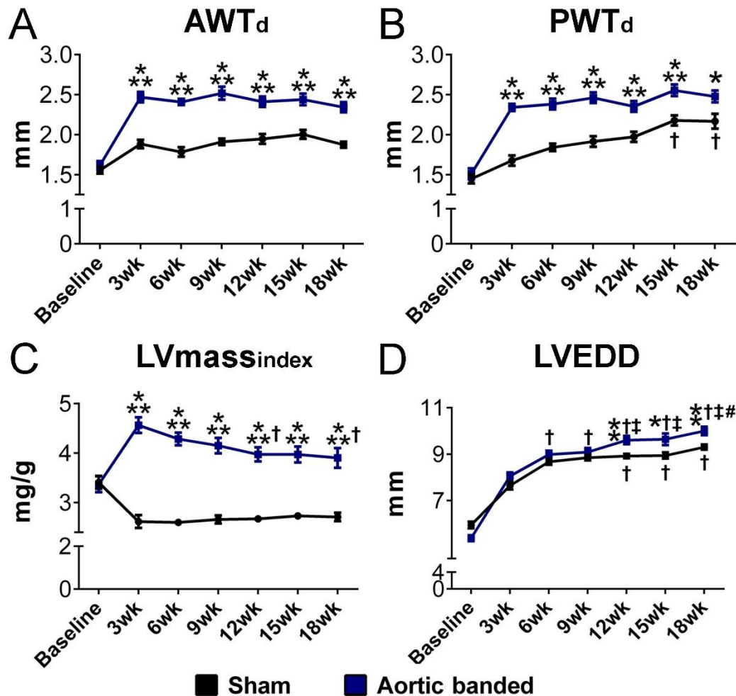
Figure 8. Echocardiographic follow-up during the development of pressure overload-induced myocardial hypertrophy. Anterior (A) and posterior (B) wall thicknesses as well as left ventricular (LV) mass index (LVmass index ) (C) were already increased after 3 weeks of LV pressure overload in the aortic banded groups. Furthermore, the aortic banded group was also associated with elevated LV end-diastolic diameter (LVEDD) (D) after 12 weeks of pressure overload. AWT d : anterior wall thickness in diastole, PWT d : posterior wall thickness in diastole *: P<0.05 vs. corresponding sham. **: P<0.01 vs. corresponding sham. ***: P<0.001 vs. corresponding sham. †: P<0.05 vs. week 3. ‡: P<0.05 vs. week 6. #: P<0.05 vs. week 9.
