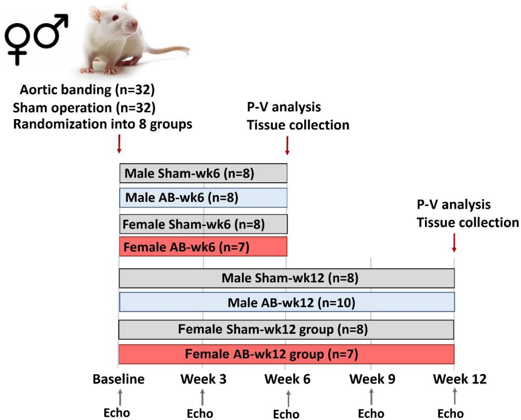
Figure 6. Schematic illustration of the experimental protocol of Study 3. At baseline, male and female rats underwent abdominal aortic banding ([AB]; n=32) or sham operation (n=32) and were subsequently randomized into 8 groups. In the male sham-wk6 (n=8) and AB-wk6 (n=8) groups and female sham-wk6 (n=8) and AB-wk6 (n=7) groups pressure-volume (P-V) analysis and tissue collection were performed at week 6. In the male sham-wk12 (n=8) and AB-wk12 (n=10) groups and female sham-wk12 (n=8) and AB-wk12 (n=7) groups pressure-volume (P-V) analysis and tissue collection were performed at week 12. Furthermore, repetitive echocardiographic measurements were performed in the male and female sham-wk12 and AB-wk12 groups.
