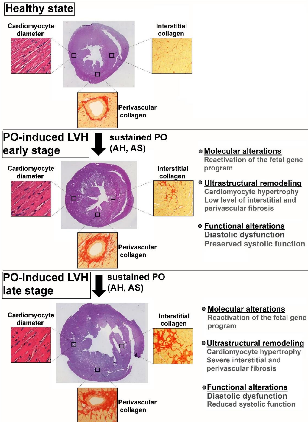
Figure 1. Summary of pressure overload-induced pathological myocardial remodeling. The early stage of pressure overload (PO)-induced left ventricular myocardial hypertrophy (LVH) is associated with cardiomyocyte hypertrophy and low level of interstitial and perivascular fibrosis on the ultrastructural level. At this stage, diastolic dysfunction is often present, however systolic function is preserved. At later stages, further accumulation of interstitial and perivascular collagen occurs. In addition, systolic function also deteriorates. AH: arterial hypertension, AS: aortic stenosis, PO: pressure overload. Cross sectional whole heart pictures are adapted from Ruppert et al. (2018) Front Physiol , 9:1869.(68)
