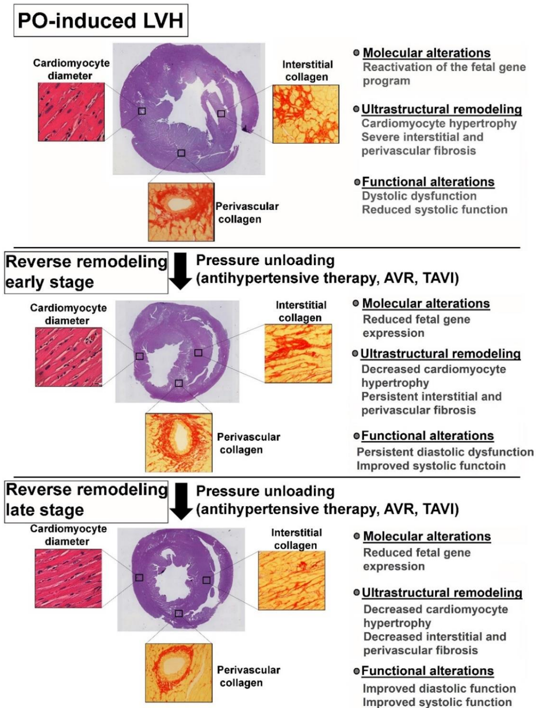
Figure 2. Summary of pressure unloading-induced myocardial reverse remodeling. Pressure unloading induces a rapid regression of cardiomyocyte hypertrophy leading to substantial reduction in left ventricular mass. However, reactive interstitial and perivascular myocardial fibrosis often persists at a relatively early stage after pressure unloading. From a functional point of view, the early phase of reverse remodeling is characterized by improved systolic function but impaired diastolic function. In contrast, at later stages, reactive myocardial fibrosis also regresses, resulting in the amelioration of diastolic function. AVR: aortic valve replacement, TAVI: transcatheter aortic valve implantation. Cross sectional whole heart pictures are adapted from Ruppert et al. (2018) Front Physiol , 9:1869.(68)
