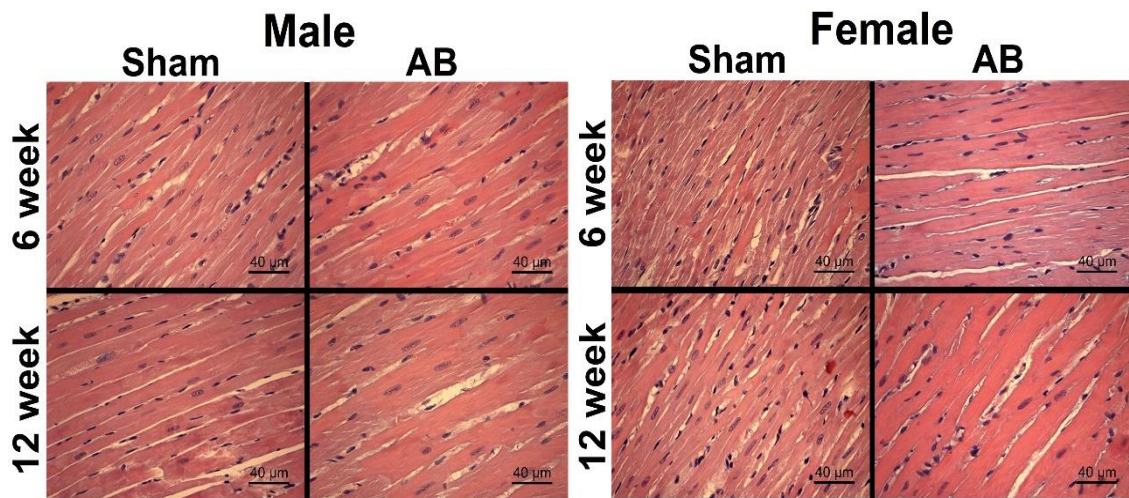
Figure 36. Representative photomicrographs demonstrating enlargement of cardiomyocytes in the aortic banded (AB) male and female groups at week 6 and 12. Hematoxylin and eosin (magnification 200x, scale bar: 40 \mu m)-stained sections are shown. AB indicates aortic banding.
