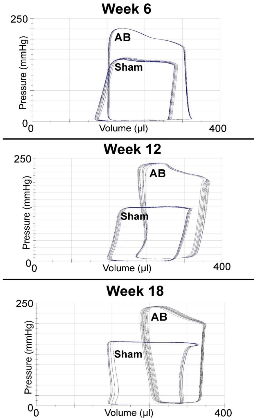
Figure 12. Representative steady-state pressure-volume (P-V) loops are shown demonstrating in vivo left ventricular (LV) function in sham and aortic banded (AB) rats at different time points. The width of the P-V loops in the AB group at week 6 does not differ from the control's width. In contrast, at week 12 and 18, the width of the loops becomes substantially smaller in the AB groups, suggesting impaired systolic performance. Furthermore, the P-V loops demonstrate a rightward shift in the AB groups at week 12 and 18, indicating chamber dilatation.
