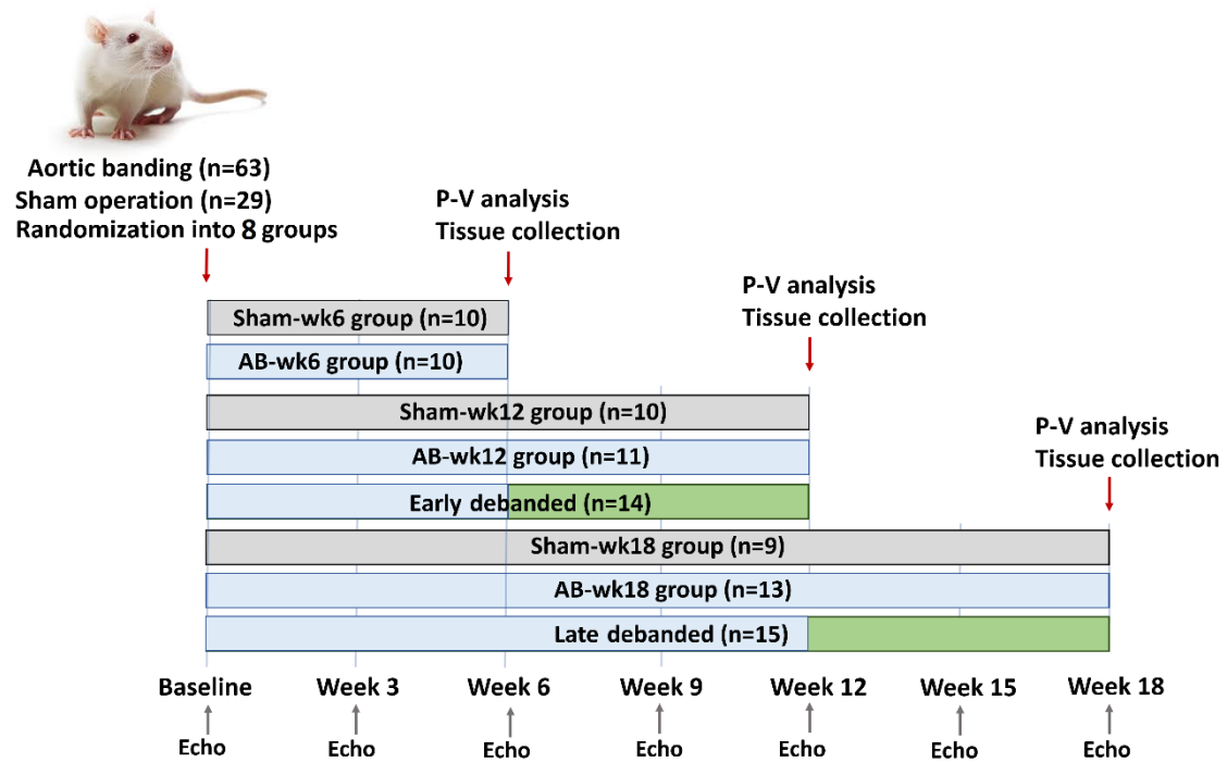
Figure 5. Schematic illustration of the experimental protocol of Study 2. At baseline, the rats underwent abdominal aortic banding ([AB]; n=63) or sham operation (n=29) and were subsequently randomized into 8 groups. The Sham-wk6 (n=10), AB-wk6 (n=10) groups were followed-up for 6 weeks. The Sham-wk12 (n=10), AB-wk12 (n=11) groups were followed-up for 12 weeks, while the Sham-wk18 (n=9), AB-wk18 (n=13) were followed-up for 18 weeks. In the early debanded group (n=14) the aortic constriction was removed after week 6, while in the late debanded group (n=15) the narrowing suture was removed after week 12.
