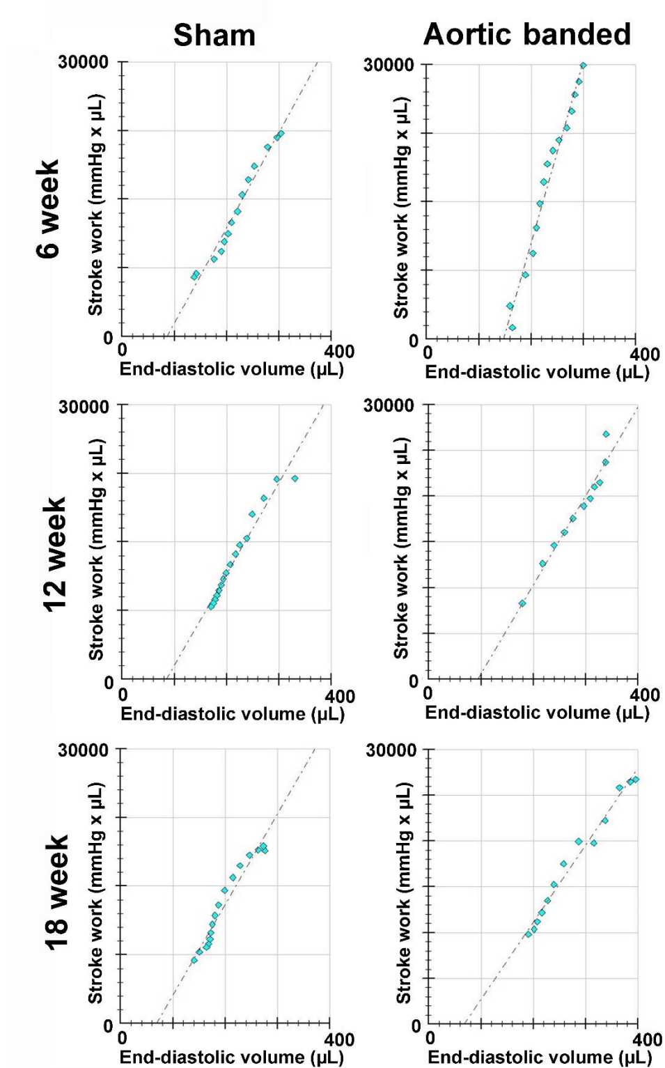
Figure 14. Alterations in preload recruitable stroke work (PRSW) during the progression of pressure overload-induced myocardial hypertrophy. PRSW indicated increased left ventricular (LV) contractility in the aortic banded (AB) group at week 6 compared to the corresponding sham group. The contractility augmentation diminished in the AB groups at week 12 and 18.
