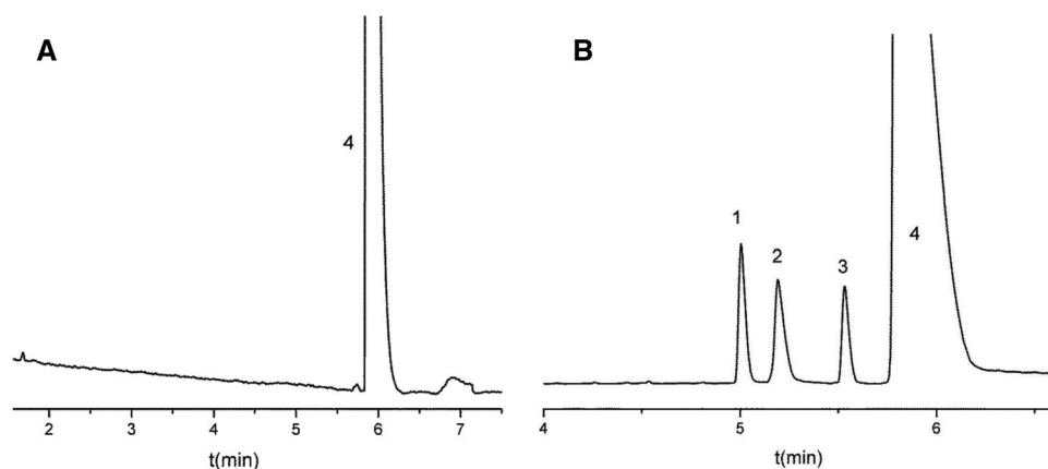
Figure 2. Representative electropherograms recorded for the Sunosi ® sample solution (A) and the sample solution spiked with impurities (B) (CE conditions: 45 mM Tris-acetate buffer, pH 4.5, 4 mM S- \gamma -CD; 200 nm, 21°C, 19.5 kV, 1: S -phenylalaninol, 2: R -phenylalaninol, 3: S -solriamfetol, 4: R -solriamfetol, 0.1% impurities in 5000 \mu g/mL R -solriamfetol sample solution).
