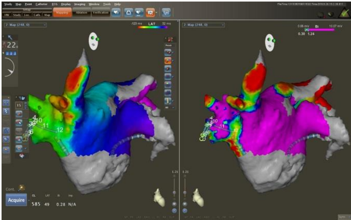
Figure 2. Atrial tachycardia after previous pulmonary vein isolation. Electroanatomical activation map (left side) and voltage map (right side) of the left atrium, performed with the CARTO system and CT-Merge. The AT originates from the right superior pulmonary vein; the site of reconnection is at the infero-anterior part of the vein. Electrophysiology Laboratory, Heart and Vascular Center, Semmelweis University.
