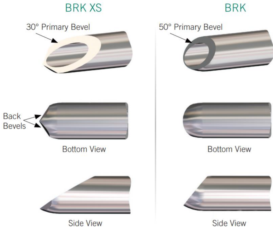
Figure 13. The difference between the tip of BRK-1 XS (left side) and BRK-1 (right side) needle is shown in the picture. The BRK-1 XS has a sharp ending, thus enabling better engagement at the targeted part of the oval fossa and making an easier breakthrough possible (Abbott Medical, EP catalog).
