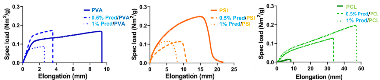
Figure 22.: Specific load-elongation curves of fibrous Pred-containing PVA, PSI, and PCL meshes (KT2).
