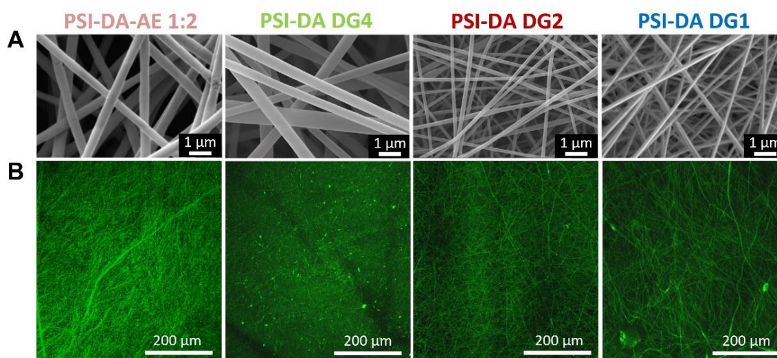
Figure 18.: SEM (A) and two-photon microscopic images (B) of fibrous PSI-DA conjugates image. (Scale bars: 1 \mu\text{m} (A); 200 \mu\text{m} (B)) (KT1).
