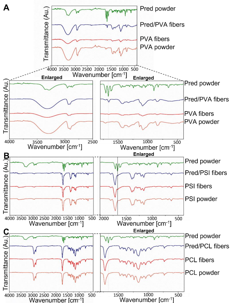
Figure 14.: FT-IR spectra of neat and Pred-containing PVA (A), PSI (B), and PCL (C) (KT2).
