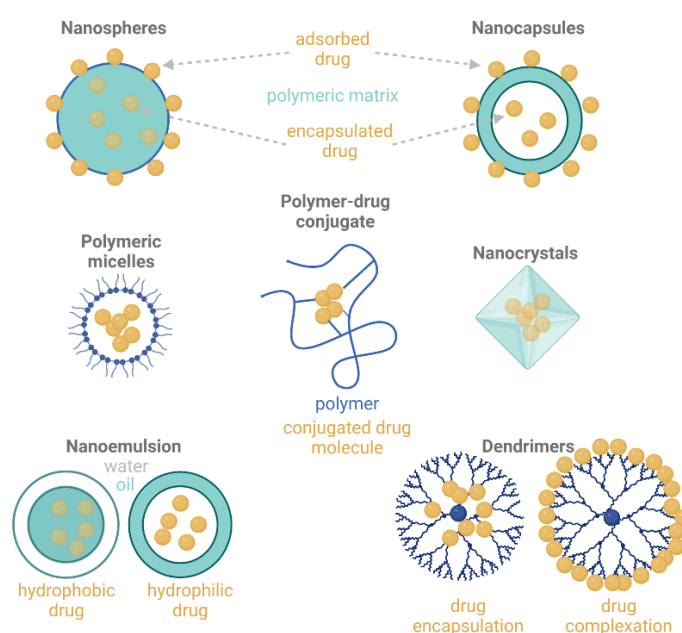
Figure 1.: Polymeric nanoformulations. The image was made by Biorender based on the work of Viswanthen et al. (12).
