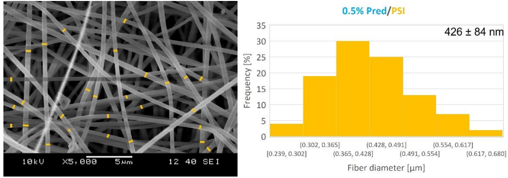
Figure 7.: Average fiber diameter of fibrous 0.5% Pred/PSI sample (KT2).
