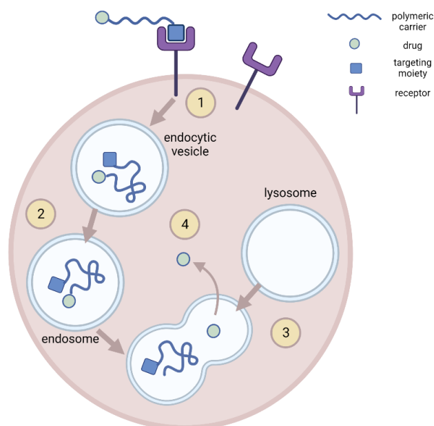
Figure 2.: Receptor-mediated internalization of polymer-drug conjugates: (1) interaction of targeting moiety and receptor, internalization; (2) transport; (3) fusion with lysosomes; (4) degradation and drug release. The image was made by Biorender based on the work of Khandare et al. (14).
