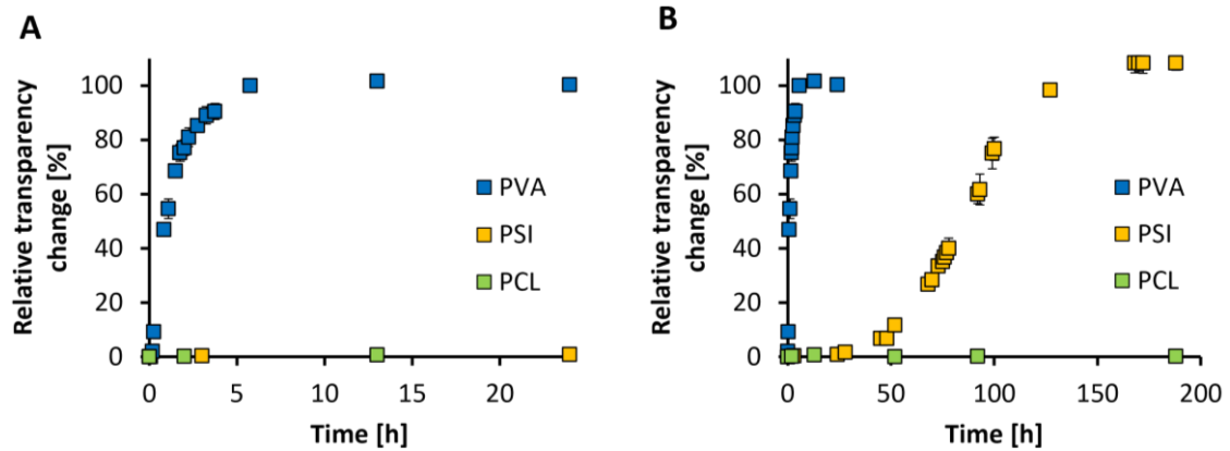
Figure 23.: Disintegration of neat PVA, PSI, and PCL meshes after 188 h (A) and 24 h (B) (KT2).
