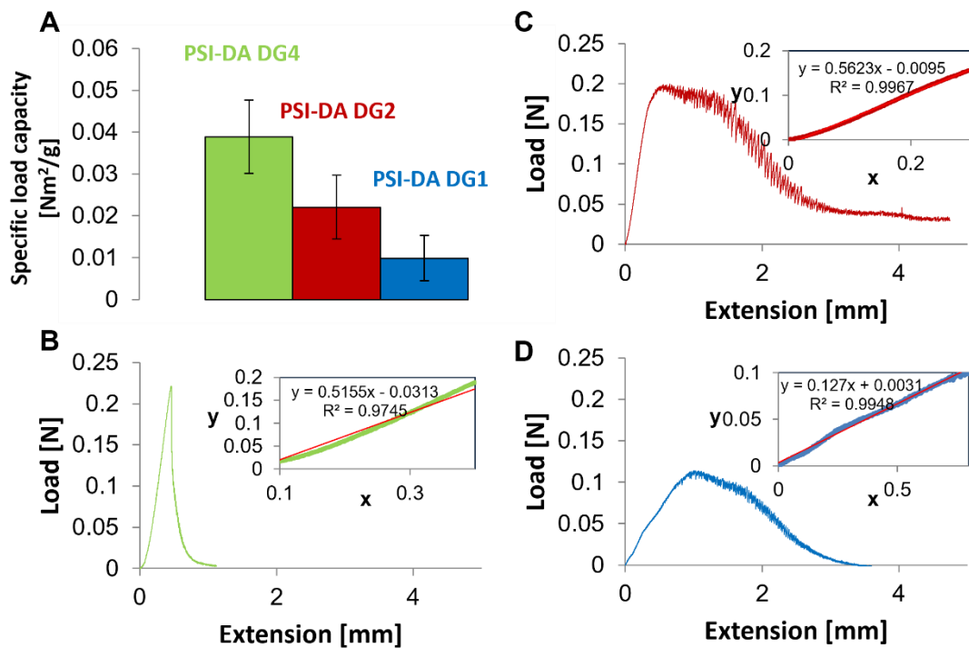
Figure 21.: Specific load capacity (A) and typical load-extension curves (C; B; D) of fibrous PSI-DA membranes with the fitted line to the initial linear ascendant period of the curves used for the determination of the initial modulus ( x : extension [mm]; y : load [N]) ( KT1 ).
