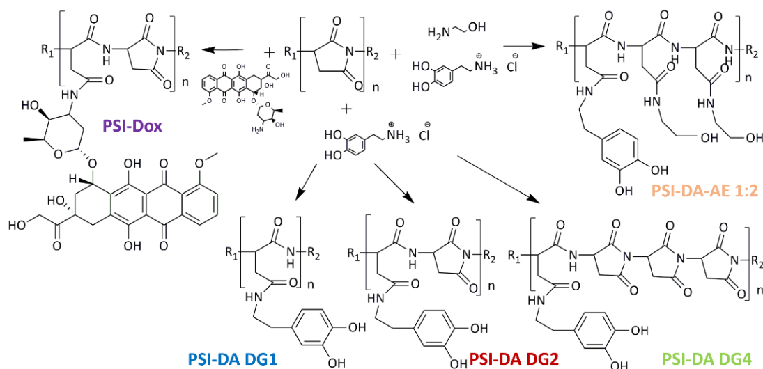
Figure 5.: Chemical composition of different PSI-DA conjugates and the PSI-Dox conjugate. R_1 : NH_2 group; R_2 : COOH group; n : repeating unit ( KT1 and KT2 ). The image was made by ChemDraw.
