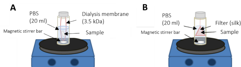
Figure 11.: Drug release setup in the case of PSI-Dox conjugate (A) and drug-loaded polymer samples (B) (KT2).
