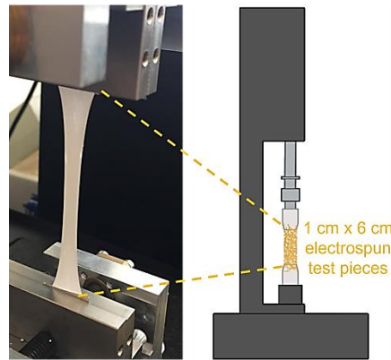
Figure 8.: Set-up for unidirectional strain-controlled mechanical tests.
