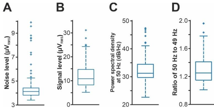
Figure 21. Quality assessment of cortical recordings ( n = 109 ). (a) Distribution of the root mean square (RMS) noise levels estimated from the recordings. (b) Distribution of the estimated RMS signal levels. (c) Distribution of power spectral density values measured at 50 Hz to demonstrate power line noise contamination (see also panel d of Fig. 19). (d) Distribution of the ratios of the power spectral density value measured at 50 Hz to the power spectral density value computed at a nearby frequency (49 Hz) without power line noise contamination.
