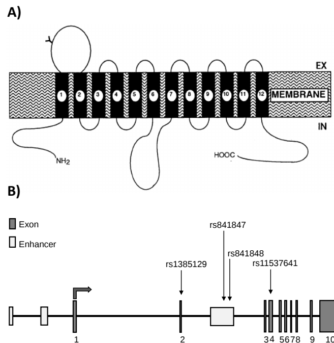
Figure 2. Schematic representation of the GLUT1 membrane protein and the coding SLC2A1 gene.
