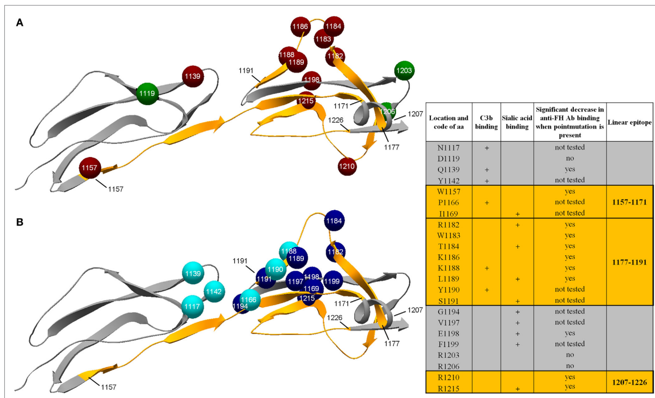
FIGURE 4 | Folded structure of complement factor H (FH) short consensus repeat domains 19–20. Panels represent the ribbon model of the molecule obtained from the Protein Data Bank (pdb2g7). Linear epitopes of the FH autoantibodies are highlighted with orange [amino acid (aa)1157–1171, aa1177–1191, and aa1207–1226], where the initial and final aa of each segment is indicated with black numbers. Arrowheads point toward the C-terminal end of the proteins. (A) The location of the generated point mutations is displayed as colorful spheres on the backbone of the protein, with white numbers indicating their location and colors their effect on autoantibody binding by FH (red: significantly decreased binding when the aa substitutions is present; green: no significant effect on binding). (B) Colorful spheres refer to aa forming the C3b (14, 35) (light blue) and sialic acid (15) (dark blue) binding sites of the molecule. Numbers within the spheres show the location of each aa.
