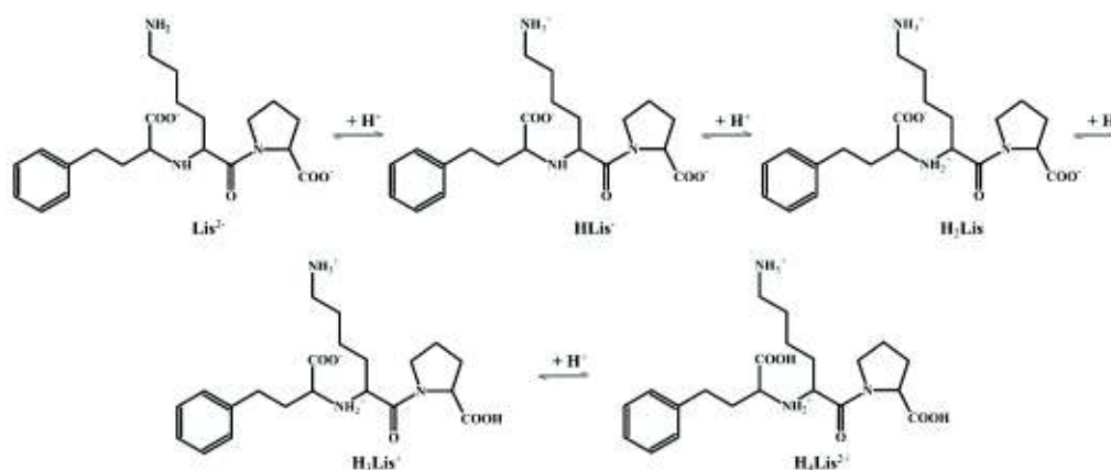
Figure 2. Stepwise protonation equilibria of lisinopril
