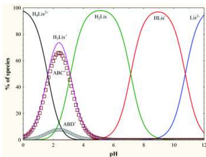
Figure 7. Distribution curves of the macrospecies ( H_4Lis ) and microspecies ( ABC and ABD ) of lisinopril
