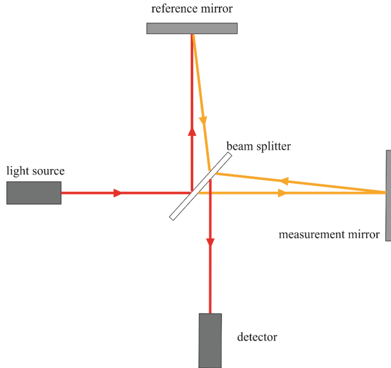
Figure 4.: Schematic drawing of a Michelson interferometer. A light source emits a low coherent light passes through a beam splitter (half-silvered mirror). One light beam is projected on a mirror at a known distance (reference arm). The other beam is measured at the test object with unknown distance. Both reflected beams pass through the beam splitter again and the created interference is captured by a detector. (Authors own image)
