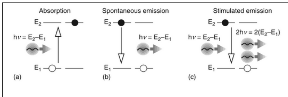
Figure 1.: Changes in quantum systems after an interaction with electromagnetic radiation. a) material absorbing the energy of a photon ( E=h\nu ( h Planck constant, \nu frequency)) moves from its ground state ( E_1 ) to an excited state ( E_2 ). b) spontaneous emission occurs after the lifetime of the excited material expires. The material returns to its original ground state, and a photon is emitted with the same energy as the difference between the excited and ground states of the material ( E_2 - E_1 ). c) Stimulated emission happens when a photon irradiates material already in excited state. During stimulated emission the material returns to its ground state, and in the mean while two photons with the same energy ( E_2 - E_1 ), same direction and same phase is emitted. 8
