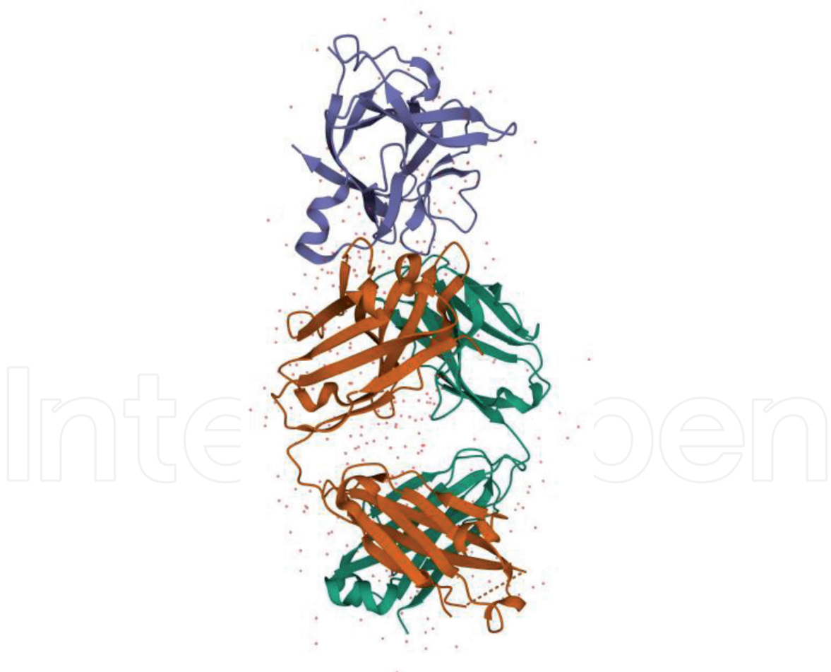
Figure 2. The IL-1 \beta structure including an \alpha -helix, \beta -sheets and loops (shown in violet color) (PDB ID 7CHZ) [38].
